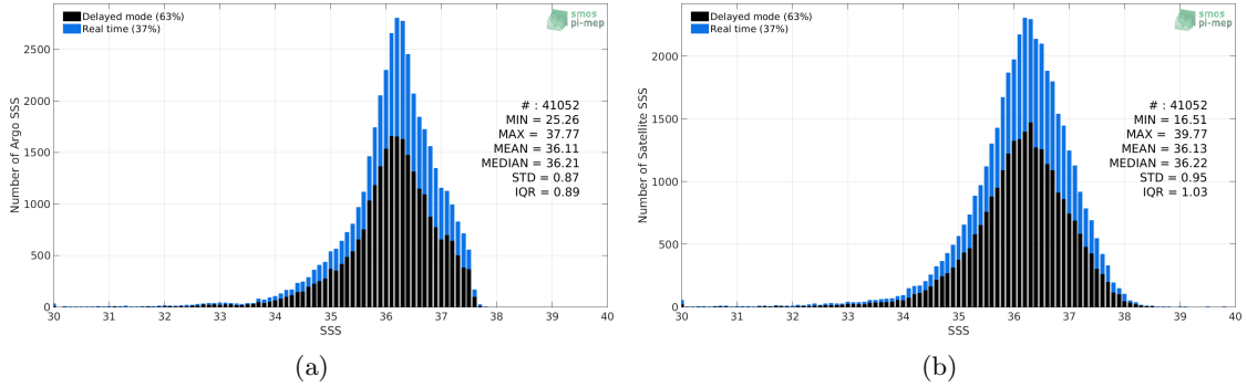
Figure 2: Histograms of SSS from Argo (a) and SMAP SSS L2 v4 (RSS) (b) considering all match-up pairs per bins of 0.1 over the Tropical Atlantic Ocean Pi-MEP region and for the full satellite product period.
