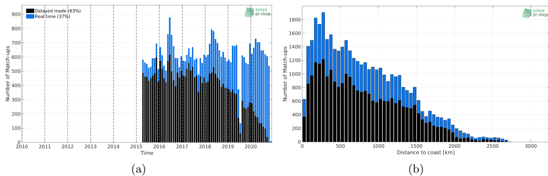
Figure 1: Number of match-ups between Argo and SMAP SSS L2 v4 (RSS) SSS as a function of time (a) and as function of the distance to coast (b) over the Tropical Atlantic Ocean Pi-MEP region and for the full satellite product period.
