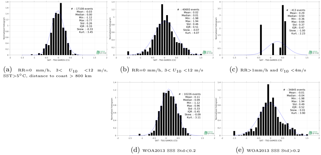
Figure 13: Normalized histogram of \Delta SSS (SMAP-L2-RSS-V3-70KM - TSG-SAMOS) for 5 different subdatasets corresponding to: RR=0 mm/h, 3 < U_{10} < 12 m/s, SST>5°C, distance to coast > 800 km (a), RR=0 mm/h, 3 < U_{10} < 12 m/s (b), RR>1mm/h and U_{10} < 4 m/s (c), WOA2013 SSS Std<0.2 (d), WOA2013 SSS Std>0.2 (e).
