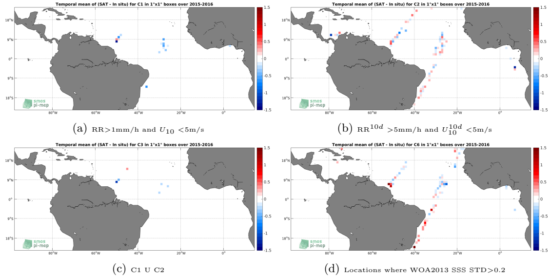
Figure 12: Temporal mean gridded over spatial boxes of size 1^\circ \times 1^\circ of \Delta\text{SSS} (SMAP-L2-RSS-V3-70KM - TSG-LEGOS-DM) for 4 different subdatasets corresponding to: RR > 1mm/h and U_{10} < 5\text{m/s} (a), \text{RR}^{10d} > 5\text{mm/h} and U_{10}^{10d} < 5\text{m/s} (b), C1 U C2 (c), Locations where WOA2013 SSS STD > 0.2 (d).
