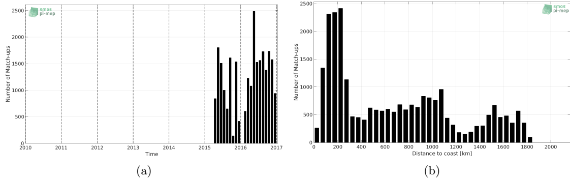
Figure 1: Number of match-ups between TSG-LEGOS-DM and SMAP-L2-RSS-V3-70KM SSS as a function of time (a) and as function of the distance to coast (b) over the Tropical Atlantic Ocean Pi-MEP region and for the full satellite product period.
