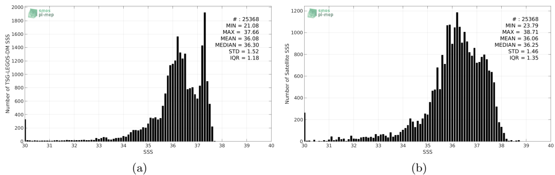
Figure 2: Histograms of SSS from TSG-LEGOS-DM (a) and SMAP-L2-RSS-V3-70KM (b) considering all match-up pairs per bins of 0.1 over the Tropical Atlantic Ocean Pi-MEP region and for the full satellite product period.
