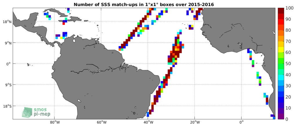
Figure 4: Number of SSS match-ups between TSG-LEGOS-DM SSS and the SMAP-L2-RSS-V3-70KM SSS product for the Tropical Atlantic Ocean Pi-MEP region over 1^\circ \times 1^\circ boxes and for the full satellite product period.
