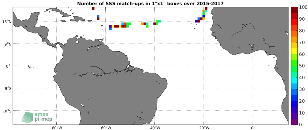
Figure 4: Number of SSS match-ups between TSG-GOSUD-Sailing-ship SSS and the SMAP-L2-RSS-V3-70KM SSS product for the Tropical Atlantic Ocean Pi-MEP region over 1^\circ \times 1^\circ boxes and for the full satellite product period.
