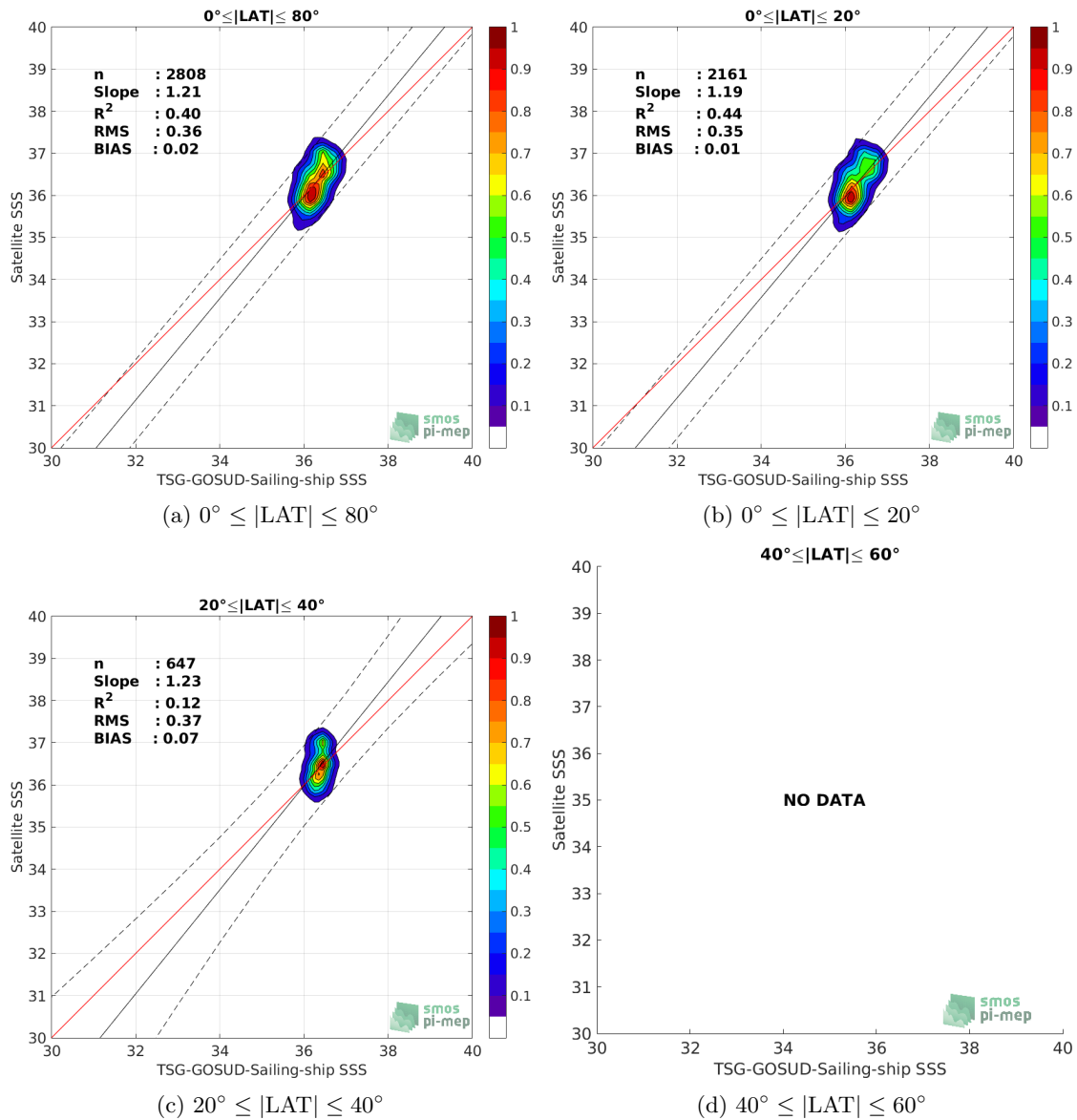
Figure 9: Contour maps of the concentration of SMAP-L2-RSS-V3-70KM SSS (y-axis) versus TSG-GOSUD-Sailing-ship SSS (x-axis) at match-up pairs for different latitude bands. For each plot, the red line shows x=y . The black thin and dashed lines indicate a linear fit through the data cloud and the \pm 95\% confidence levels, respectively. The number match-up pairs n , the slope and R^2 coefficient of the linear fit, the root mean square (RMS) and the mean bias between satellite and in situ data are indicated for each latitude band in each plot.
