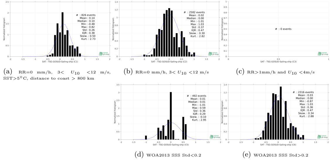
Figure 13: Normalized histogram of \Delta SSS (SMAP-L2-RSS-V3-70KM - TSG-GOSUD-Sailing-ship) for 5 different subdatasets corresponding to: RR=0 mm/h, 3 < U_{10} < 12 m/s, SST>5°C, distance to coast > 800 km (a), RR=0 mm/h, 3 < U_{10} < 12 m/s (b), RR>1mm/h and U_{10} < 4 m/s (c), WOA2013 SSS Std<0.2 (d), WOA2013 SSS Std>0.2 (e).
