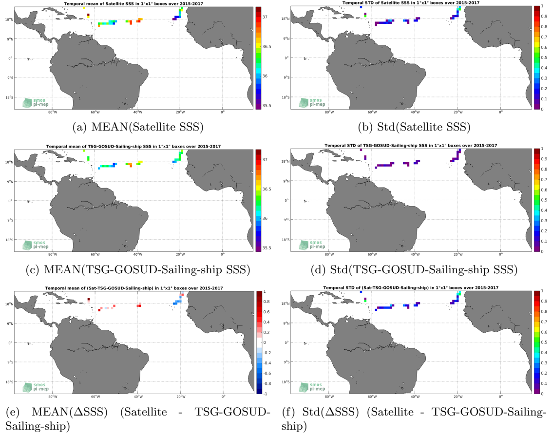
Figure 6: Temporal mean (left) and Std (right) of SSS from SMAP-L2-RSS-V3-70KM (top), TSG-GOSUD-Sailing-ship (middle), and of \Delta SSS (Satellite - TSG-GOSUD-Sailing-ship). Only match-up pairs are used to generate these maps.
