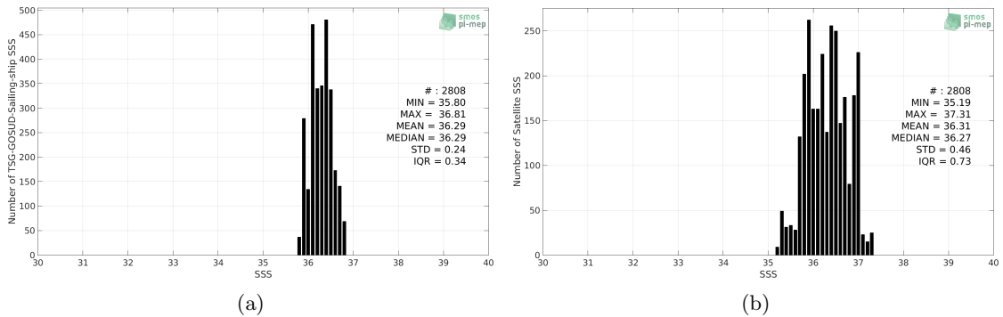
Figure 2: Histograms of SSS from TSG-GOSUD-Sailing-ship (a) and SMAP-L2-RSS-V3-70KM (b) considering all match-up pairs per bins of 0.1 over the Tropical Atlantic Ocean Pi-MEP region and for the full satellite product period.
