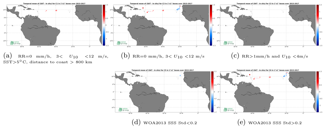
Figure 12: Temporal mean gridded over spatial boxes of size 1^\circ \times 1^\circ of \Delta SSS (SMAP-L2-RSS-V3-70KM - TSG-GOSUD-Sailing-ship) for 5 different subdatasets corresponding to:RR=0 mm/h, 3 < U_{10} < 12 m/s, SST >5^\circ C, distance to coast > 800 km (a), RR=0 mm/h, 3 < U_{10} < 12 m/s (b), RR >1 mm/h and U_{10} < 4 m/s (c), WOA2013 SSS Std <0.2 (d), WOA2013 SSS Std >0.2 (e).
