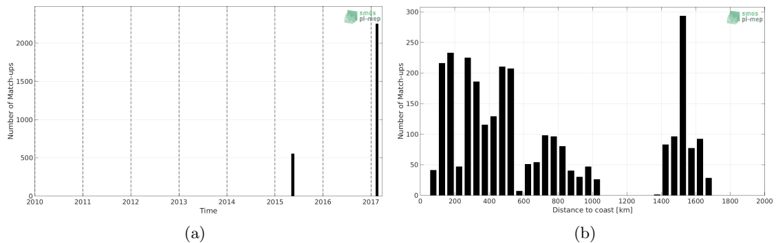
Figure 1: Number of match-ups between TSG-GOSUD-Sailing-ship and SMAP-L2-RSS-V3-70KM SSS as a function of time (a) and as function of the distance to coast (b) over the Tropical Atlantic Ocean Pi-MEP region and for the full satellite product period.
