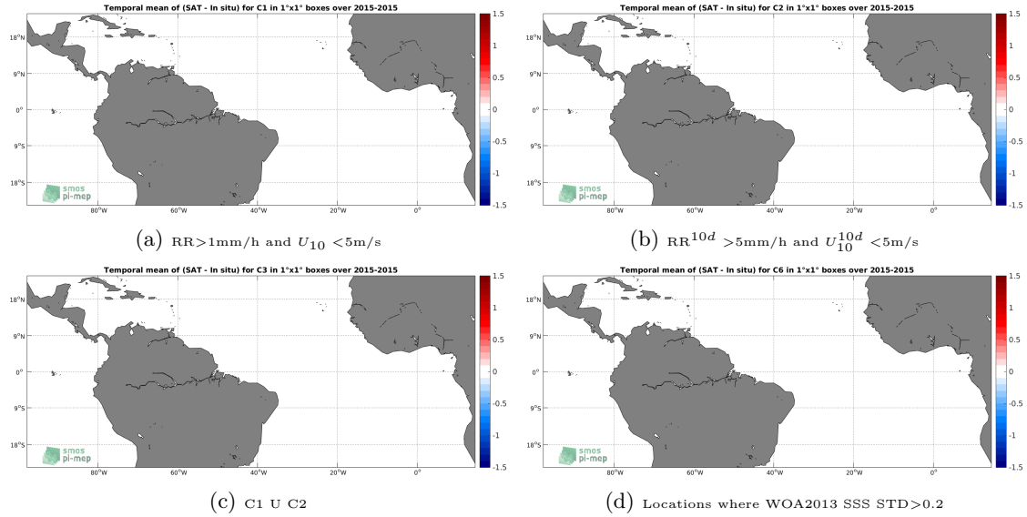
Figure 12: Temporal mean gridded over spatial boxes of size 1^\circ \times 1^\circ of \Delta SSS (SMAP-L2-RSS-V3-70KM - TSG-GOSUD-Sailing-ship) for 4 different subdatasets corresponding to:RR > 1 mm/h and U_{10} < 5 m/s (a), RR^{10d} > 5 mm/h and U_{10}^{10d} < 5 m/s (b), C1 U C2 (c),Locations where WOA2013 SSS STD > 0.2 (d).
