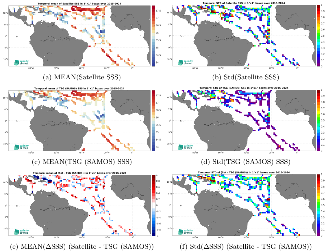
Figure 7: Temporal mean (left) and Std (right) of SSS from SMAP SSS L2 v5.0 (JPL) (top), TSG (SAMOS) (middle), and of \Delta SSS (Satellite - TSG (SAMOS)). Only match-up pairs are used to generate these maps.
