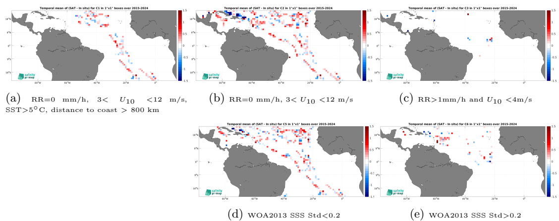
Figure 14: Temporal mean gridded over spatial boxes of size 1^\circ \times 1^\circ of \Delta\text{SSS} (SMAP SSS L2 v5.0 (JPL) - TSG (SAMOS)) for 5 different subdatasets corresponding to:RR=0 mm/h, 3 < U_{10} < 12 m/s, SST >5^\circ\text{C} , distance to coast > 800 km (a), RR=0 mm/h, 3 < U_{10} < 12 m/s (b), RR >1 mm/h and U_{10} < 4 m/s (c), WOA2013 SSS Std <0.2 (d), WOA2013 SSS Std >0.2 (e).
