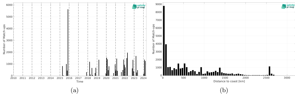
Figure 2: Number of match-ups between TSG (SAMOS) and SMAP SSS L2 v5.0 (JPL) SSS as a function of time (a) and as function of the distance to coast (b) over the Tropical Atlantic Ocean Pi-MEP region and for the full satellite product period.
