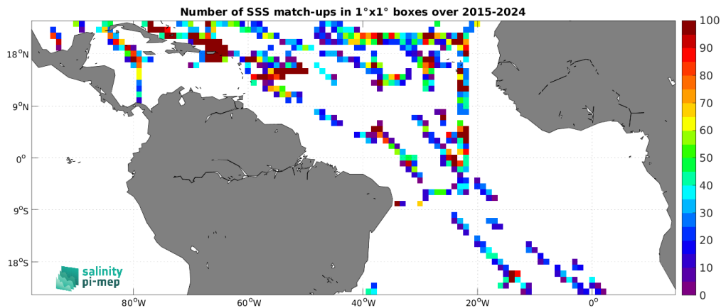
Figure 5: Number of SSS match-ups between TSG (SAMOS) SSS and the SMAP SSS L2 v5.0 (JPL) SSS product for the Tropical Atlantic Ocean Pi-MEP region over 1^\circ \times 1^\circ boxes and for the full satellite product period.
