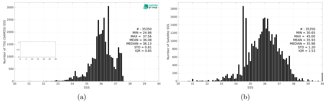
Figure 3: Histograms of SSS from TSG (SAMOS) (a) and SMAP SSS L2 v5.0 (JPL) (b) considering all match-up pairs per bins of 0.1 over the Tropical Atlantic Ocean Pi-MEP region and for the full satellite product period.
