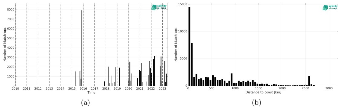
Figure 1: Number of match-ups between TSG (SAMOS) and SMAP SSS L2 v5.0 (JPL) SSS as a function of time (a) and as function of the distance to coast (b) over the Tropical Atlantic Ocean Pi-MEP region and for the full satellite product period.
