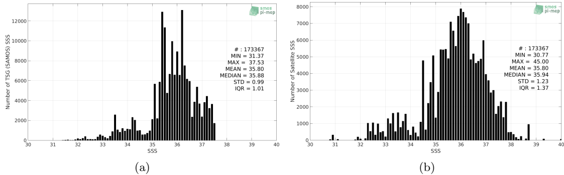
Figure 2: Histograms of SSS from TSG (SAMOS) (a) and SMAP SSS L2 v5.0 (JPL) (b) considering all match-up pairs per bins of 0.1 over the Tropical Atlantic Ocean Pi-MEP region and for the full satellite product period.
