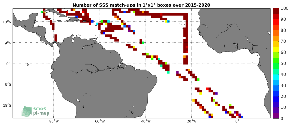
Figure 4: Number of SSS match-ups between TSG (SAMOS) SSS and the SMAP SSS L2 v5.0 (JPL) SSS product for the Tropical Atlantic Ocean Pi-MEP region over 1°x1° boxes and for the full satellite product period.
