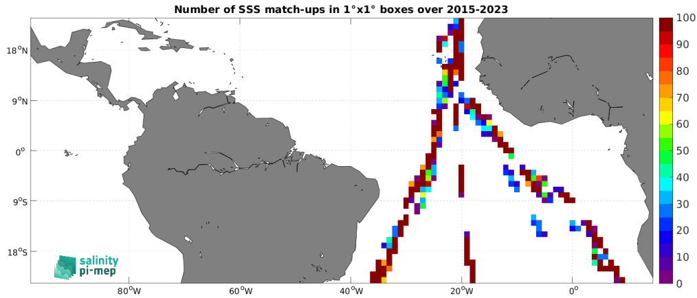
Figure 5: Number of SSS match-ups between TSG (Polarstern) SSS and the SMAP SSS L2 v5.0 (JPL) SSS product for the Tropical Atlantic Ocean Pi-MEP region over 1^\circ \times 1^\circ boxes and for the full satellite product period.
