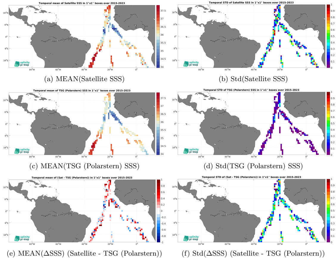
Figure 7: Temporal mean (left) and Std (right) of SSS from SMAP SSS L2 v5.0 (JPL) (top), TSG (Polarstern) (middle), and of \Delta\text{SSS} (Satellite - TSG (Polarstern)). Only match-up pairs are used to generate these maps.
