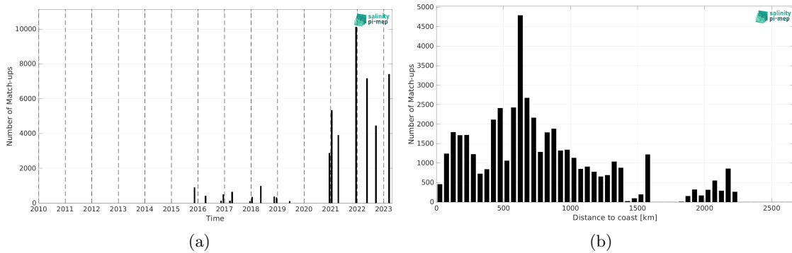
Figure 2: Number of match-ups between TSG (Polarstern) and SMAP SSS L2 v5.0 (JPL) SSS as a function of time (a) and as function of the distance to coast (b) over the Tropical Atlantic Ocean Pi-MEP region and for the full satellite product period.
