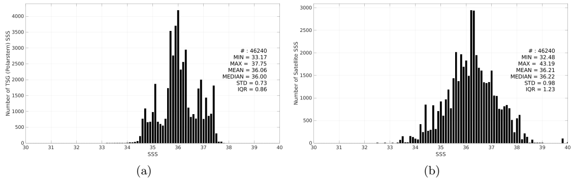
Figure 3: Histograms of SSS from TSG (Polarstern) (a) and SMAP SSS L2 v5.0 (JPL) (b) considering all match-up pairs per bins of 0.1 over the Tropical Atlantic Ocean Pi-MEP region and for the full satellite product period.
