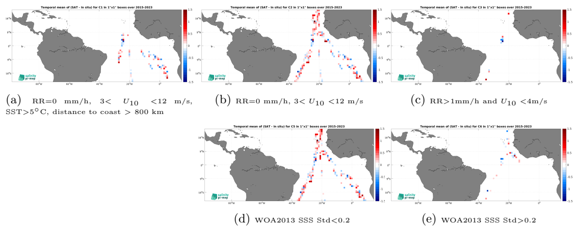
Figure 14: Temporal mean gridded over spatial boxes of size 1^\circ \times 1^\circ of \Delta\text{SSS} (SMAP SSS L2 v5.0 (JPL) - TSG (Polarstern)) for 5 different subdatasets corresponding to:RR=0 mm/h, 3 < U_{10} < 12 m/s, SST >5^\circ\text{C} , distance to coast > 800 km (a), RR=0 mm/h, 3 < U_{10} < 12 m/s (b), RR >1 mm/h and U_{10} < 4 m/s (c), WOA2013 SSS Std <0.2 (d), WOA2013 SSS Std >0.2 (e).
