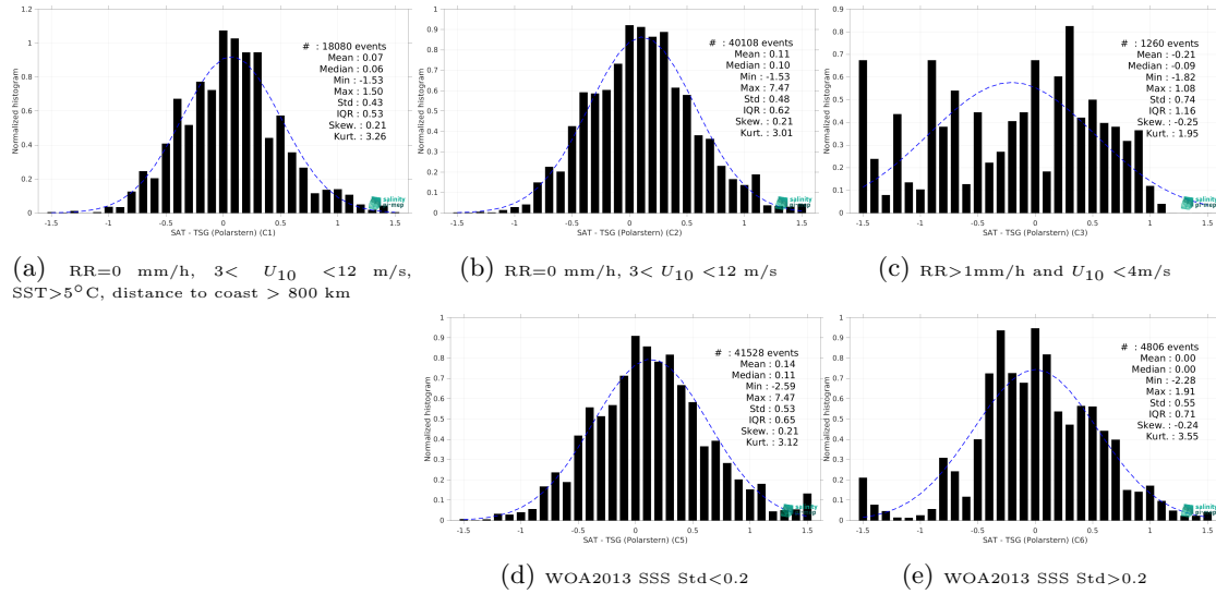
Figure 13: Normalized histogram of \Delta SSS (SMAP SSS L2 v5.0 (JPL) - TSG (Polarstern)) for 5 different subdatasets corresponding to: RR=0 mm/h, 3 < U_{10} < 12 m/s, SST > 5°C, distance to coast > 800 km (a), RR=0 mm/h, 3 < U_{10} < 12 m/s (b), RR > 1mm/h and U_{10} < 4 m/s (c), WOA2013 SSS Std < 0.2 (d), WOA2013 SSS Std > 0.2 (e).
