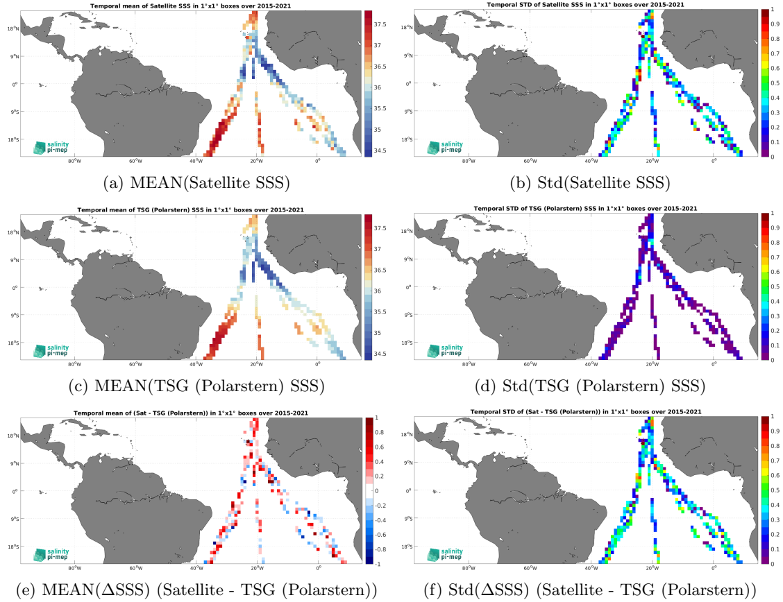
Figure 6: Temporal mean (left) and Std (right) of SSS from SMAP SSS L2 v5.0 (JPL) (top), TSG (Polarstern) (middle), and of \Delta\text{SSS} (Satellite - TSG (Polarstern)). Only match-up pairs are used to generate these maps.
