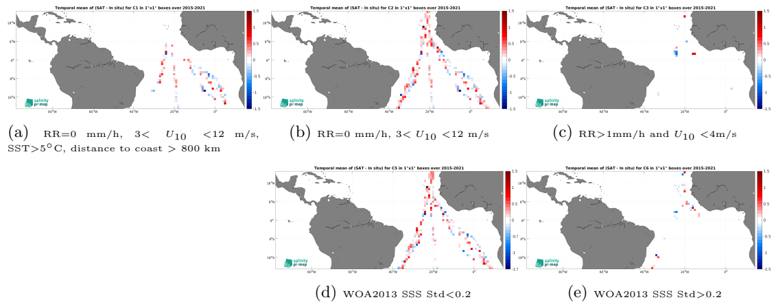
Figure 12: Temporal mean gridded over spatial boxes of size 1^\circ \times 1^\circ of \Delta\text{SSS} (SMAP SSS L2 v5.0 (JPL) - TSG (Polarstern)) for 5 different subdatasets corresponding to:RR=0 mm/h, 3 < U_{10} < 12 m/s, SST >5^\circ\text{C} , distance to coast > 800 km (a), RR=0 mm/h, 3 < U_{10} < 12 m/s (b), RR >1 mm/h and U_{10} < 4 m/s (c), WOA2013 SSS Std <0.2 (d), WOA2013 SSS Std >0.2 (e).
