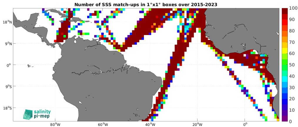
Figure 5: Number of SSS match-ups between TSG (LEGOS-DM) SSS and the SMAP SSS L2 v5.0 (JPL) SSS product for the Tropical Atlantic Ocean Pi-MEP region over 1^\circ \times 1^\circ boxes and for the full satellite product period.
