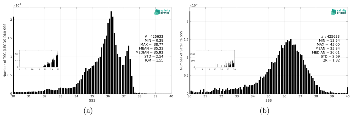
Figure 3: Histograms of SSS from TSG (LEGOS-DM) (a) and SMAP SSS L2 v5.0 (JPL) (b) considering all match-up pairs per bins of 0.1 over the Tropical Atlantic Ocean Pi-MEP region and for the full satellite product period.
