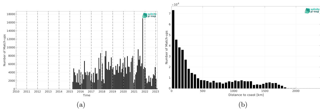
Figure 2: Number of match-ups between TSG (LEGOS-DM) and SMAP SSS L2 v5.0 (JPL) SSS as a function of time (a) and as function of the distance to coast (b) over the Tropical Atlantic Ocean Pi-MEP region and for the full satellite product period.
