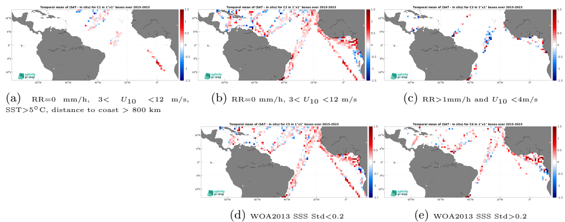
Figure 14: Temporal mean gridded over spatial boxes of size 1^\circ \times 1^\circ of \Delta SSS (SMAP SSS L2 v5.0 (JPL) - TSG (LEGOS-DM)) for 5 different subdatasets corresponding to:RR=0 mm/h, 3 < U_{10} < 12 m/s, SST >5^\circ\text{C} , distance to coast > 800 km (a), RR=0 mm/h, 3 < U_{10} < 12 m/s (b), RR >1 mm/h and U_{10} < 4 m/s (c), WOA2013 SSS Std <0.2 (d), WOA2013 SSS Std >0.2 (e).
