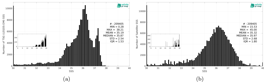
Figure 3: Histograms of SSS from TSG (LEGOS-DM) (a) and SMAP SSS L2 v5.0 (JPL) (b) considering all match-up pairs per bins of 0.1 over the Tropical Atlantic Ocean Pi-MEP region and for the full satellite product period.
