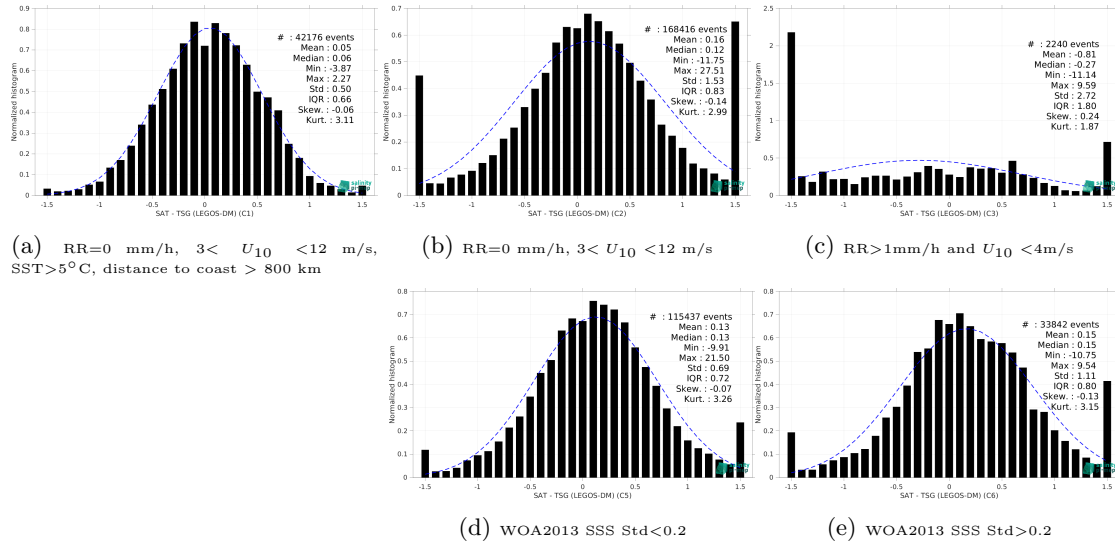
Figure 15: Normalized histogram of \Delta\text{SSS} (SMAP SSS L2 v5.0 (JPL) - TSG (LEGOS-DM)) for 5 different subdatasets corresponding to: RR=0 mm/h, 3 < U_{10} < 12 m/s, SST>5°C, distance to coast > 800 km (a), RR=0 mm/h, 3 < U_{10} < 12 m/s (b), RR>1mm/h and U_{10} < 4 m/s (c), WOA2013 SSS Std<0.2 (d), WOA2013 SSS Std>0.2 (e).
