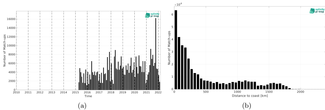
Figure 1: Number of match-ups between TSG (LEGOS-DM) and SMAP SSS L2 v5.0 (JPL) SSS as a function of time (a) and as function of the distance to coast (b) over the Tropical Atlantic Ocean Pi-MEP region and for the full satellite product period.
