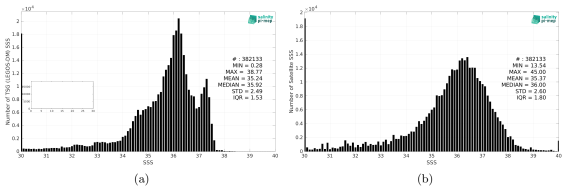
Figure 2: Histograms of SSS from TSG (LEGOS-DM) (a) and SMAP SSS L2 v5.0 (JPL) (b) considering all match-up pairs per bins of 0.1 over the Tropical Atlantic Ocean Pi-MEP region and for the full satellite product period.
