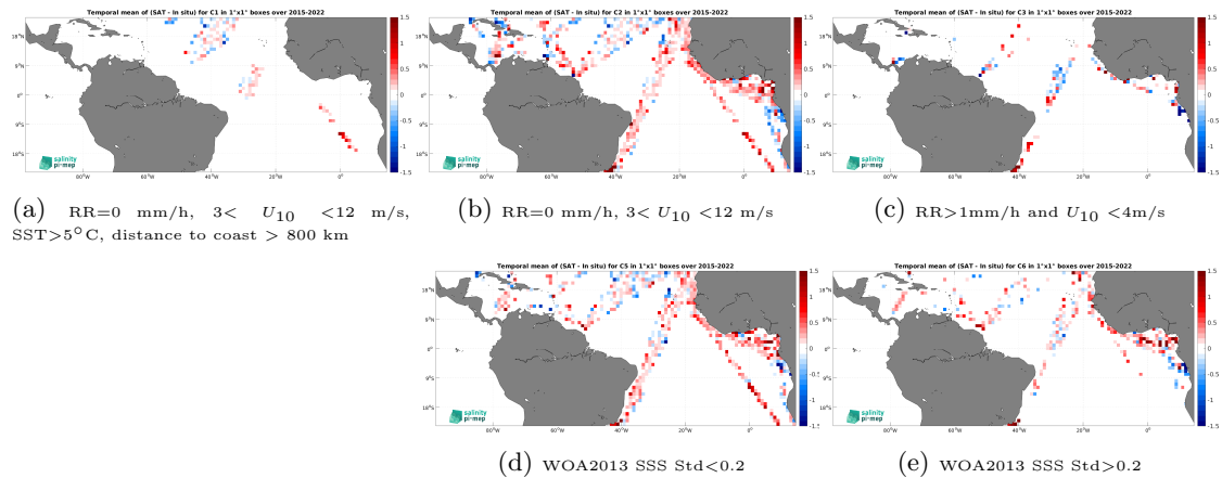
Figure 12: Temporal mean gridded over spatial boxes of size 1^\circ \times 1^\circ of \Delta\text{SSS} (SMAP SSS L2 v5.0 (JPL) - TSG (LEGOS-DM)) for 5 different subdatasets corresponding to:RR=0 mm/h, 3 < U_{10} < 12 m/s, SST >5^\circ\text{C} , distance to coast > 800 km (a), RR=0 mm/h, 3 < U_{10} < 12 m/s (b), RR >1 mm/h and U_{10} < 4 m/s (c), WOA2013 SSS Std <0.2 (d), WOA2013 SSS Std >0.2 (e).
