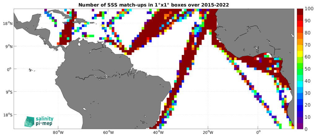
Figure 4: Number of SSS match-ups between TSG (LEGOS-DM) SSS and the SMAP SSS L2 v5.0 (JPL) SSS product for the Tropical Atlantic Ocean Pi-MEP region over 1^\circ \times 1^\circ boxes and for the full satellite product period.
