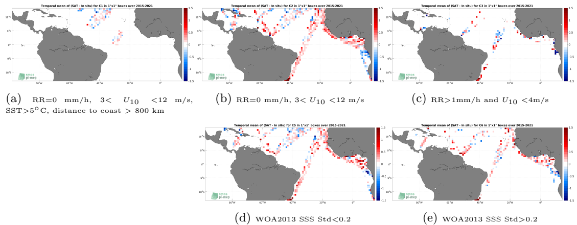
Figure 12: Temporal mean gridded over spatial boxes of size 1^\circ \times 1^\circ of \Delta SSS (SMAP SSS L2 v5.0 (JPL) - TSG (LEGOS-DM)) for 5 different subdatasets corresponding to: RR=0 mm/h, 3 < U_{10} < 12 m/s, SST > 5^\circ C , distance to coast > 800 km (a), RR=0 mm/h, 3 < U_{10} < 12 m/s (b), RR > 1 mm/h and U_{10} < 4 m/s (c), WOA2013 SSS Std < 0.2 (d), WOA2013 SSS Std > 0.2 (e).
