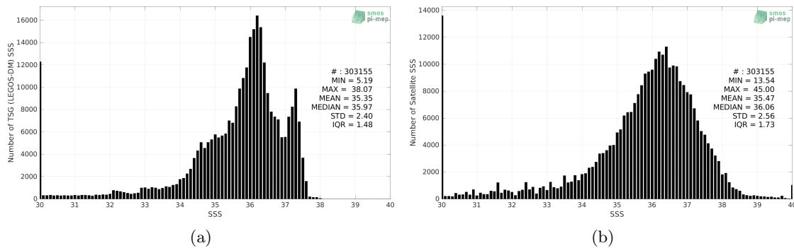
Figure 2: Histograms of SSS from TSG (LEGOS-DM) (a) and SMAP SSS L2 v5.0 (JPL) (b) considering all match-up pairs per bins of 0.1 over the Tropical Atlantic Ocean Pi-MEP region and for the full satellite product period.
