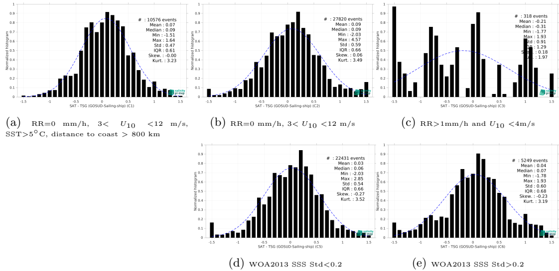
Figure 15: Normalized histogram of \Delta SSS (SMAP SSS L2 v5.0 (JPL) - TSG (GOSUD-Sailing-ship)) for 5 different subdatasets corresponding to: RR=0 mm/h, 3 < U_{10} < 12 m/s, SST>5°C, distance to coast > 800 km (a), RR=0 mm/h, 3 < U_{10} < 12 m/s (b), RR>1mm/h and U_{10} < 4 m/s (c), WOA2013 SSS Std<0.2 (d), WOA2013 SSS Std>0.2 (e).
