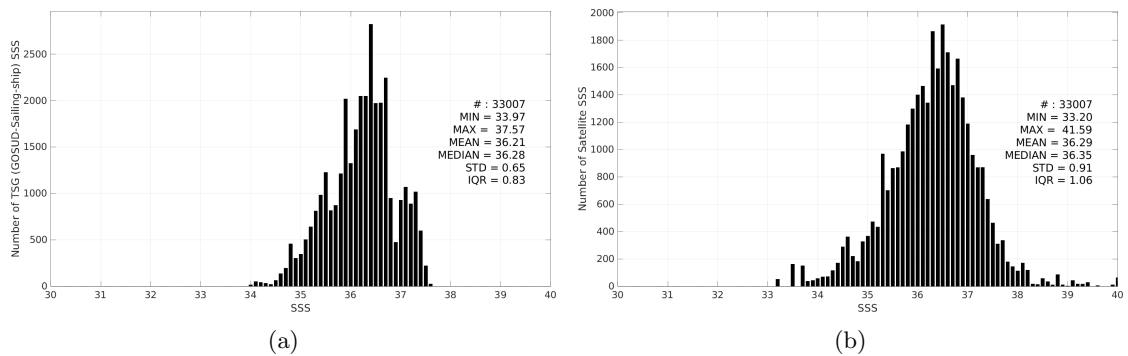
Figure 3: Histograms of SSS from TSG (GOSUD-Sailing-ship) (a) and SMAP SSS L2 v5.0 (JPL) (b) considering all match-up pairs per bins of 0.1 over the Tropical Atlantic Ocean Pi-MEP region and for the full satellite product period.
