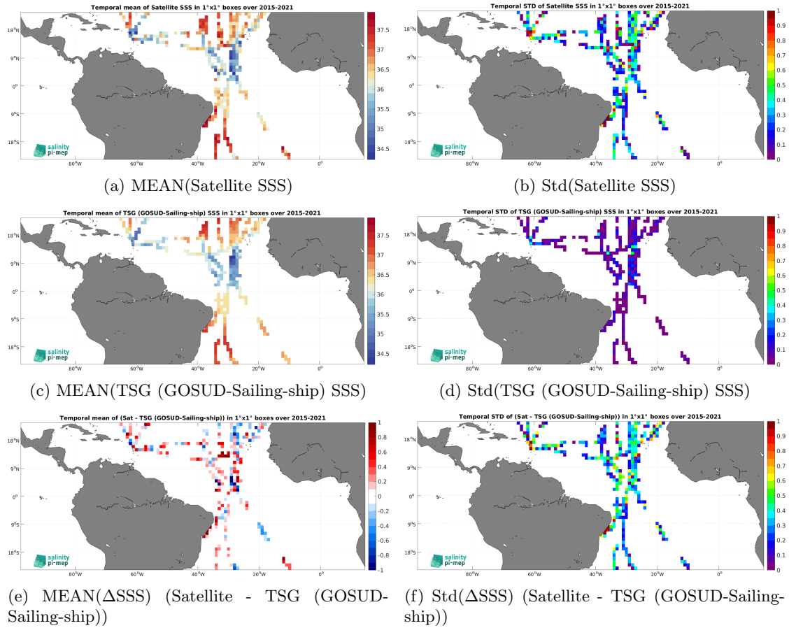
Figure 7: Temporal mean (left) and Std (right) of SSS from SMAP SSS L2 v5.0 (JPL) (top), TSG (GOSUD-Sailing-ship) (middle), and of \Delta SSS (Satellite - TSG (GOSUD-Sailing-ship)). Only match-up pairs are used to generate these maps.
