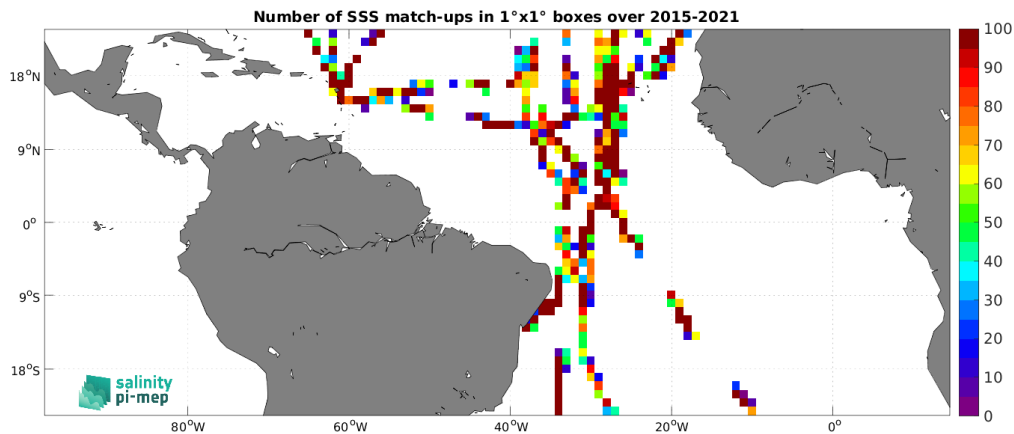
Figure 5: Number of SSS match-ups between TSG (GOSUD-Sailing-ship) SSS and the SMAP SSS L2 v5.0 (JPL) SSS product for the Tropical Atlantic Ocean Pi-MEP region over 1^\circ \times 1^\circ boxes and for the full satellite product period.
