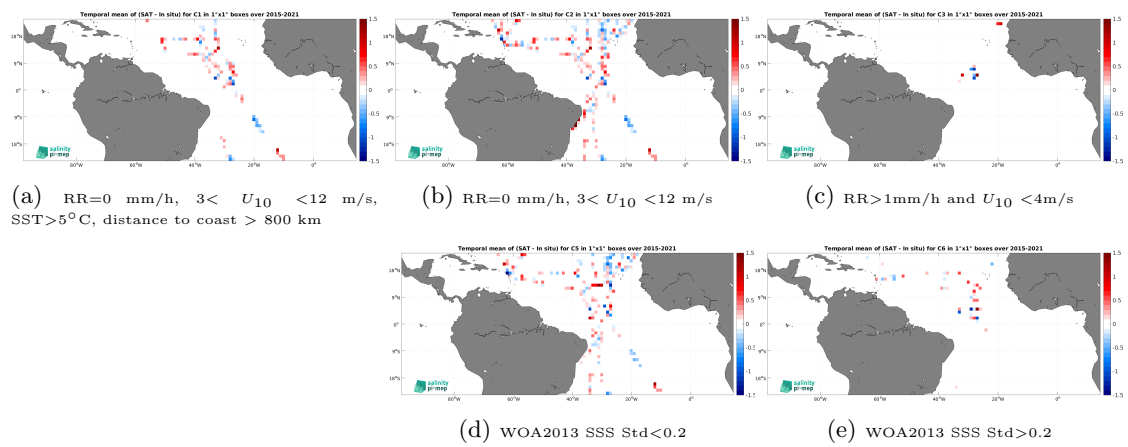
Figure 14: Temporal mean gridded over spatial boxes of size 1^\circ \times 1^\circ of \Delta\text{SSS} (SMAP SSS L2 v5.0 (JPL) - TSG (GOSUD-Sailing-ship)) for 5 different subdatasets corresponding to:RR=0 mm/h, 3 < U_{10} < 12 m/s, SST >5^\circ\text{C} , distance to coast > 800 km (a), RR=0 mm/h, 3 < U_{10} < 12 m/s (b), RR >1 mm/h and U_{10} < 4 m/s (c), WOA2013 SSS Std <0.2 (d), WOA2013 SSS Std >0.2 (e).
