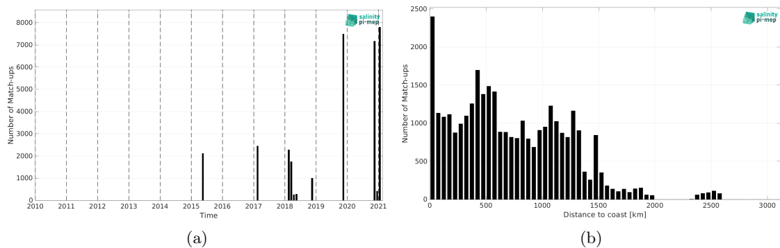
Figure 2: Number of match-ups between TSG (GOSUD-Sailing-ship) and SMAP SSS L2 v5.0 (JPL) SSS as a function of time (a) and as function of the distance to coast (b) over the Tropical Atlantic Ocean Pi-MEP region and for the full satellite product period.
