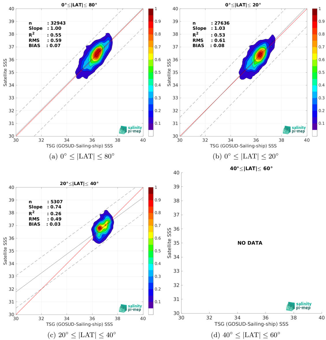
Figure 10: Contour maps of the concentration of SMAP SSS L2 v5.0 (JPL) SSS (y-axis) versus TSG (GOSUD-Sailing-ship) SSS (x-axis) at match-up pairs for different latitude bands. For each plot, the red line shows x=y . The black thin and dashed lines indicate a linear fit through the data cloud and the \pm 95\% confidence levels, respectively. The number match-up pairs n , the slope and R^2 coefficient of the linear fit, the root mean square (RMS) and the mean bias between satellite and in situ data are indicated for each latitude band in each plots.
