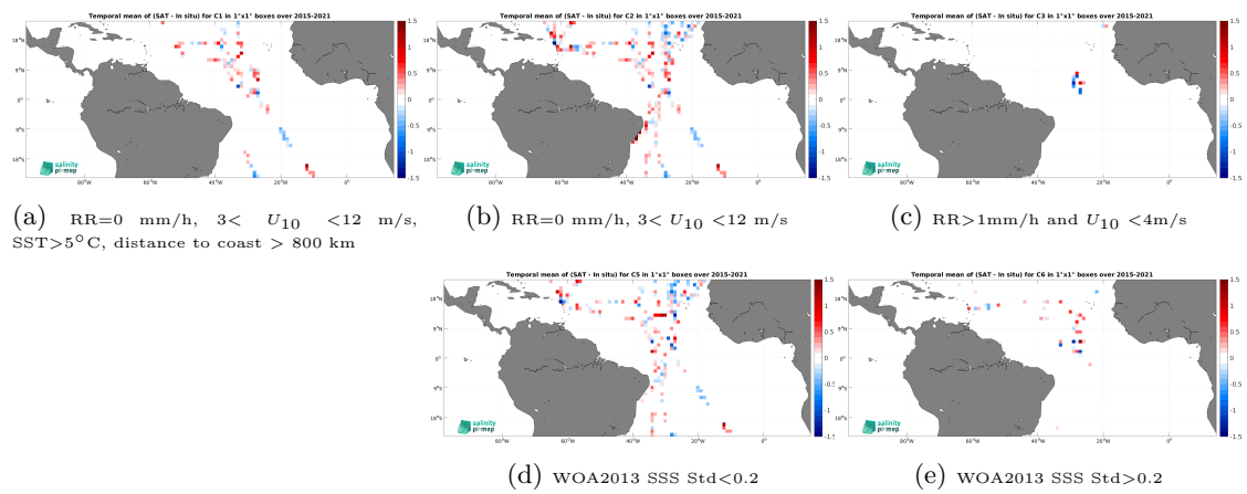
Figure 12: Temporal mean gridded over spatial boxes of size 1^\circ \times 1^\circ of \Delta\text{SSS} (SMAP SSS L2 v5.0 (JPL) - TSG (GOSUD-Sailing-ship)) for 5 different subdatasets corresponding to:RR=0 mm/h, 3 < U_{10} < 12 m/s, SST >5^\circ\text{C} , distance to coast > 800 km (a), RR=0 mm/h, 3 < U_{10} < 12 m/s (b), RR >1 mm/h and U_{10} < 4 m/s (c), WOA2013 SSS Std <0.2 (d), WOA2013 SSS Std >0.2 (e).
