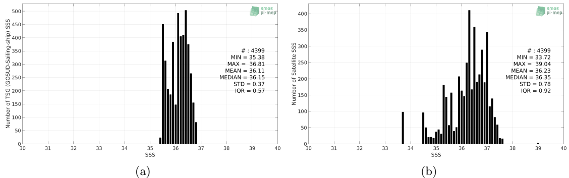
Figure 2: Histograms of SSS from TSG (GOSUD-Sailing-ship) (a) and SMAP SSS L2 v5.0 (JPL) (b) considering all match-up pairs per bins of 0.1 over the Tropical Atlantic Ocean Pi-MEP region and for the full satellite product period.
