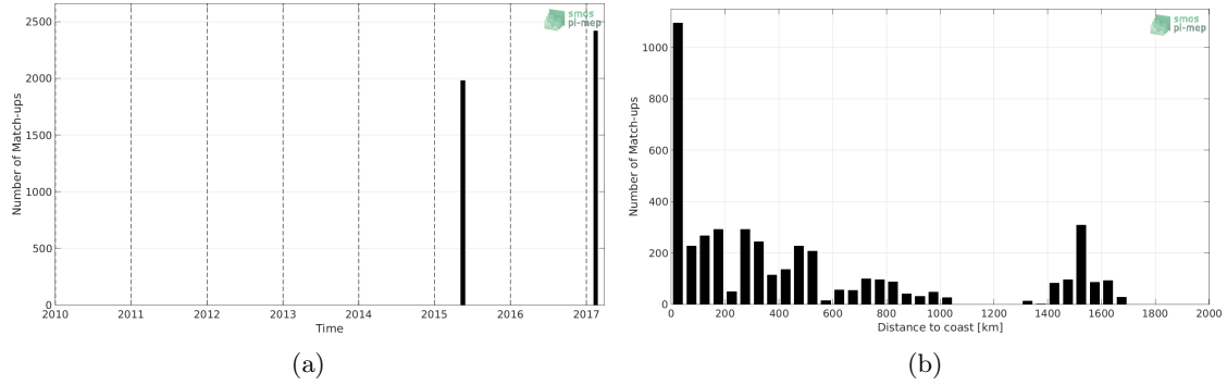
Figure 1: Number of match-ups between TSG (GOSUD-Sailing-ship) and SMAP SSS L2 v5.0 (JPL) SSS as a function of time (a) and as function of the distance to coast (b) over the Tropical Atlantic Ocean Pi-MEP region and for the full satellite product period.
