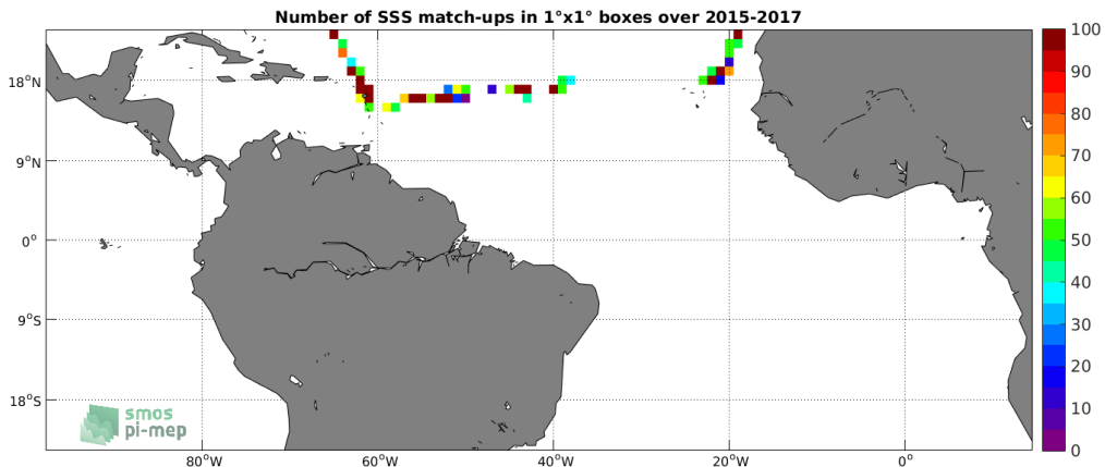
Figure 4: Number of SSS match-ups between TSG (GOSUD-Sailing-ship) SSS and the SMAP SSS L2 v5.0 (JPL) SSS product for the Tropical Atlantic Ocean Pi-MEP region over 1^\circ \times 1^\circ boxes and for the full satellite product period.
