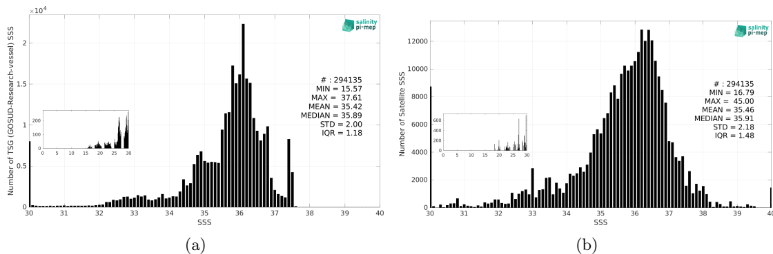
Figure 3: Histograms of SSS from TSG (GOSUD-Research-vessel) (a) and SMAP SSS L2 v5.0 (JPL) (b) considering all match-up pairs per bins of 0.1 over the Tropical Atlantic Ocean Pi-MEP region and for the full satellite product period.
