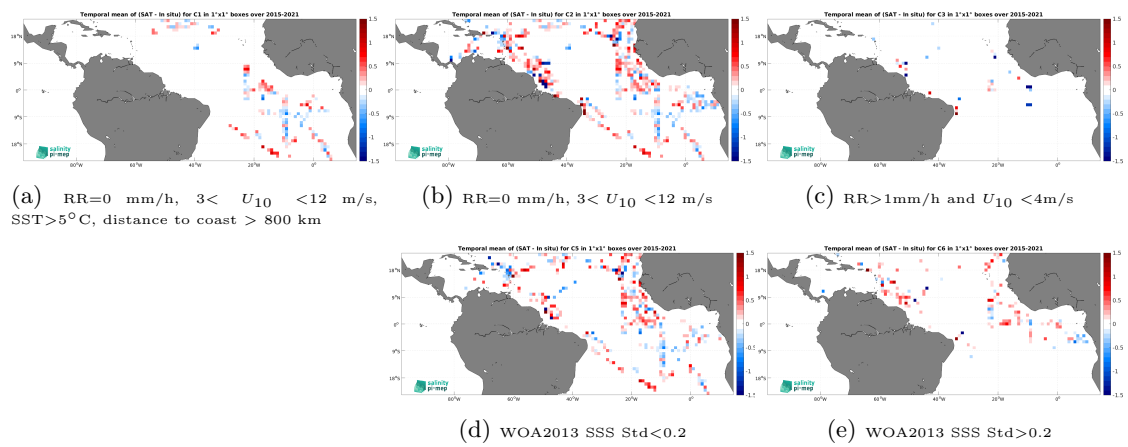
Figure 14: Temporal mean gridded over spatial boxes of size 1^\circ \times 1^\circ of \Delta SSS (SMAP SSS L2 v5.0 (JPL) - TSG (GOSUD-Research-vessel)) for 5 different subdatasets corresponding to:RR=0 mm/h, 3 < U_{10} < 12 m/s, SST>5°C, distance to coast > 800 km (a), RR=0 mm/h, 3 < U_{10} < 12 m/s (b), RR>1mm/h and U_{10} < 4 m/s (c), WOA2013 SSS Std<0.2 (d), WOA2013 SSS Std>0.2 (e).
