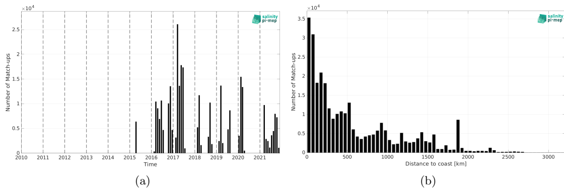
Figure 2: Number of match-ups between TSG (GOSUD-Research-vessel) and SMAP SSS L2 v5.0 (JPL) SSS as a function of time (a) and as function of the distance to coast (b) over the Tropical Atlantic Ocean Pi-MEP region and for the full satellite product period.
