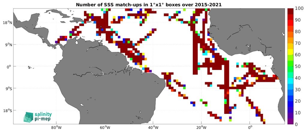
Figure 5: Number of SSS match-ups between TSG (GOSUD-Research-vessel) SSS and the SMAP SSS L2 v5.0 (JPL) SSS product for the Tropical Atlantic Ocean Pi-MEP region over 1^\circ \times 1^\circ boxes and for the full satellite product period.
