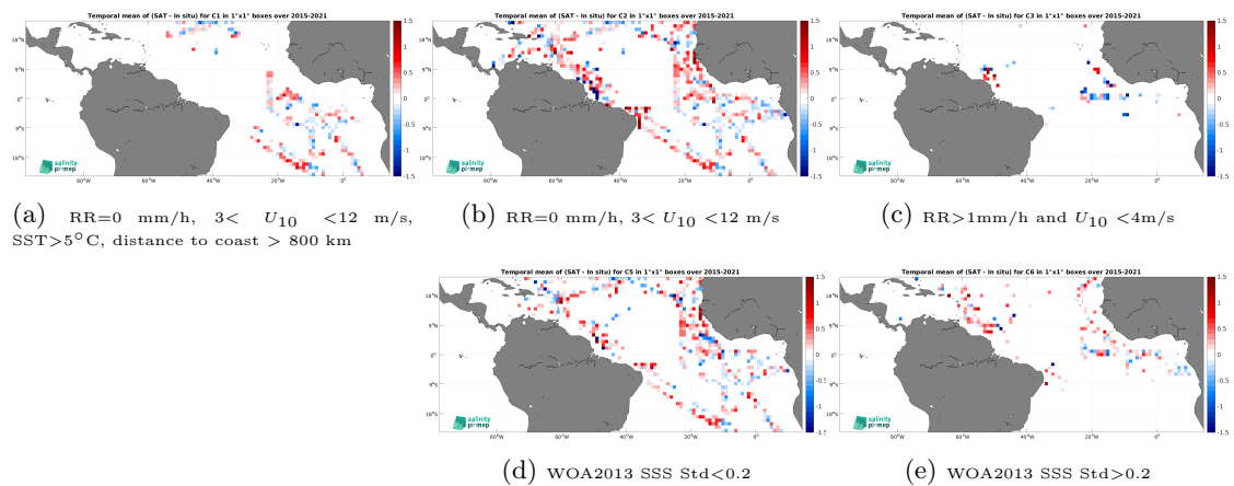
Figure 12: Temporal mean gridded over spatial boxes of size 1^\circ \times 1^\circ of \Delta\text{SSS} (SMAP SSS L2 v5.0 (JPL) - TSG (GOSUD-Research-vessel)) for 5 different subdatasets corresponding to:RR=0 mm/h, 3 < U_{10} < 12 m/s, SST>5°C, distance to coast > 800 km (a), RR=0 mm/h, 3 < U_{10} < 12 m/s (b), RR>1mm/h and U_{10} < 4 m/s (c), WOA2013 SSS Std<0.2 (d), WOA2013 SSS Std>0.2 (e).
