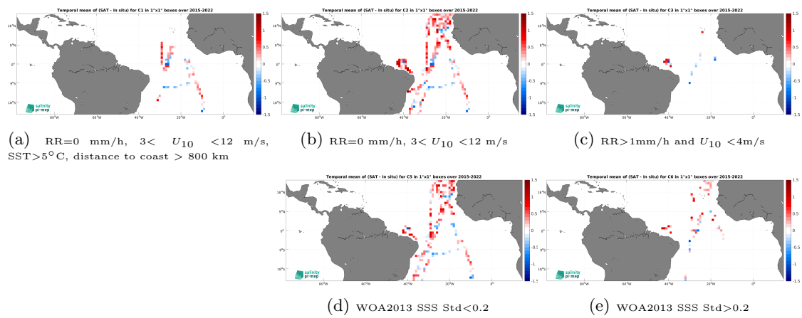
Figure 14: Temporal mean gridded over spatial boxes of size 1^\circ \times 1^\circ of \Delta SSS (SMAP SSS L2 v5.0 (JPL) - TSG (CSIC-UTM)) for 5 different subdatasets corresponding to:RR=0 mm/h, 3 < U_{10} < 12 m/s, SST >5^\circ\text{C} , distance to coast > 800 km (a), RR=0 mm/h, 3 < U_{10} < 12 m/s (b), RR >1 mm/h and U_{10} < 4 m/s (c), WOA2013 SSS Std <0.2 (d), WOA2013 SSS Std >0.2 (e).
