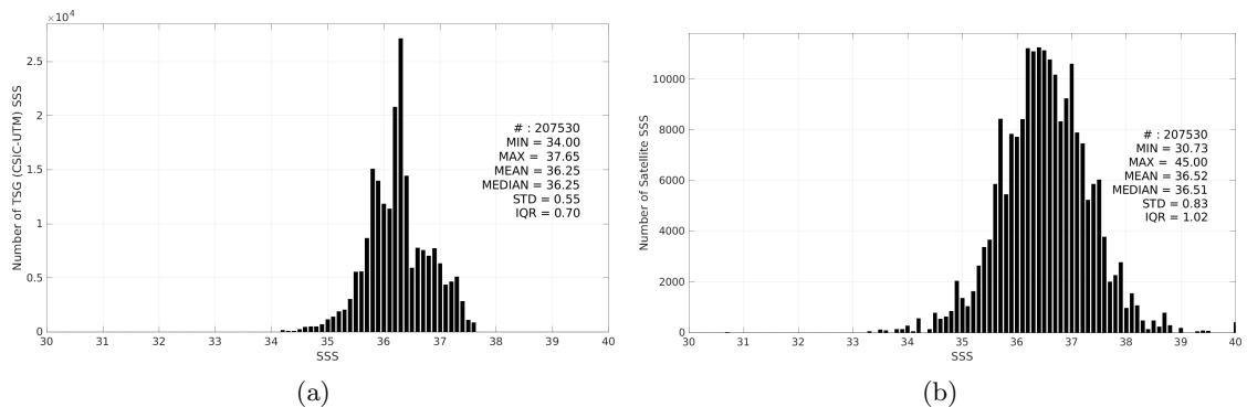
Figure 3: Histograms of SSS from TSG (CSIC-UTM) (a) and SMAP SSS L2 v5.0 (JPL) (b) considering all match-up pairs per bins of 0.1 over the Tropical Atlantic Ocean Pi-MEP region and for the full satellite product period.
