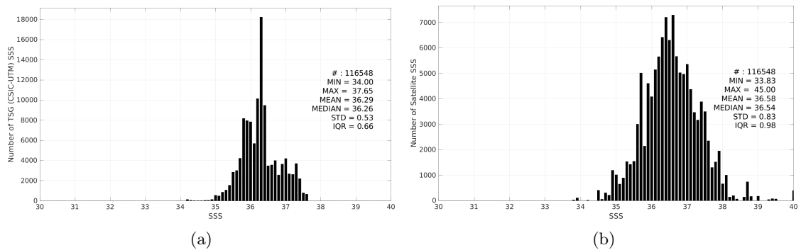
Figure 3: Histograms of SSS from TSG (CSIC-UTM) (a) and SMAP SSS L2 v5.0 (JPL) (b) considering all match-up pairs per bins of 0.1 over the Tropical Atlantic Ocean Pi-MEP region and for the full satellite product period.
