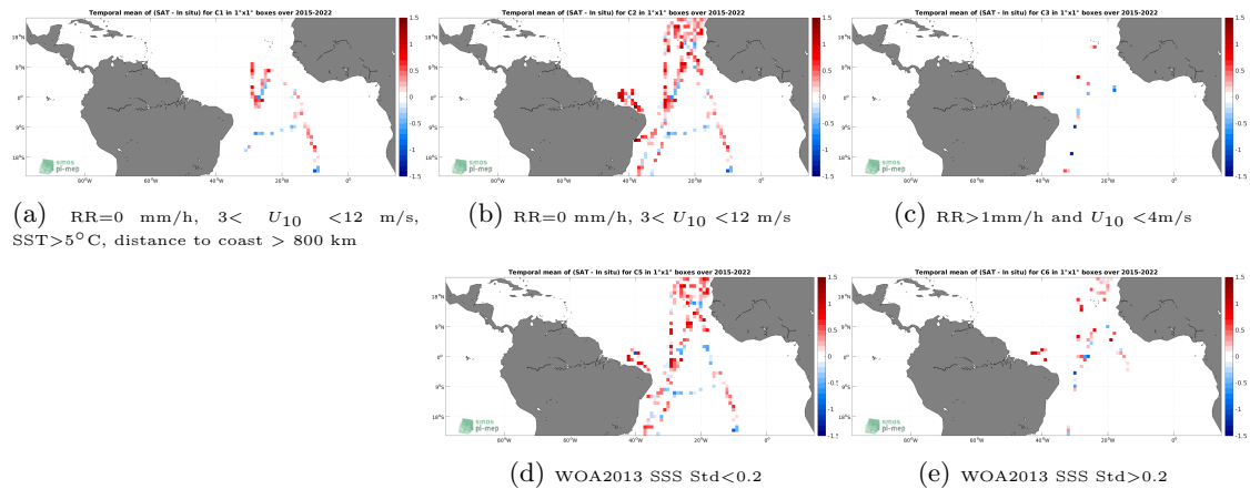
Figure 12: Temporal mean gridded over spatial boxes of size 1^\circ \times 1^\circ of \Delta\text{SSS} (SMAP SSS L2 v5.0 (JPL) - TSG (CSIC-UTM)) for 5 different subdatasets corresponding to:RR=0 mm/h, 3 < U_{10} < 12 m/s, SST >5^\circ\text{C} , distance to coast > 800 km (a), RR=0 mm/h, 3 < U_{10} < 12 m/s (b), RR >1 mm/h and U_{10} < 4 m/s (c), WOA2013 SSS Std <0.2 (d), WOA2013 SSS Std >0.2 (e).
