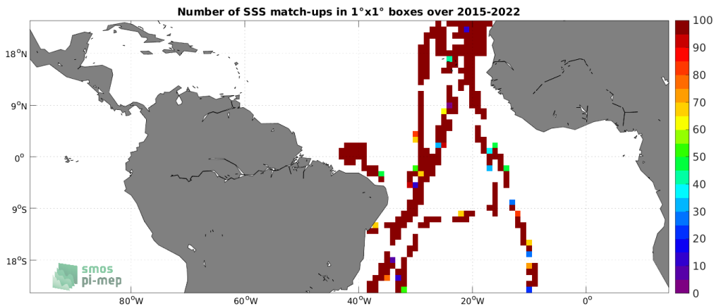
Figure 4: Number of SSS match-ups between TSG (CSIC-UTM) SSS and the SMAP SSS L2 v5.0 (JPL) SSS product for the Tropical Atlantic Ocean Pi-MEP region over 1^\circ \times 1^\circ boxes and for the full satellite product period.
