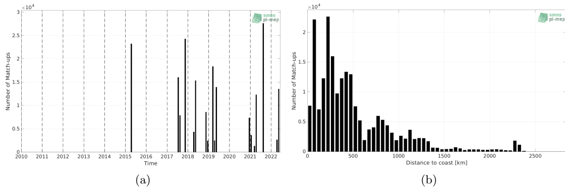
Figure 1: Number of match-ups between TSG (CSIC-UTM) and SMAP SSS L2 v5.0 (JPL) SSS as a function of time (a) and as function of the distance to coast (b) over the Tropical Atlantic Ocean Pi-MEP region and for the full satellite product period.
