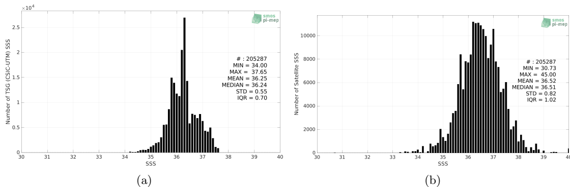
Figure 2: Histograms of SSS from TSG (CSIC-UTM) (a) and SMAP SSS L2 v5.0 (JPL) (b) considering all match-up pairs per bins of 0.1 over the Tropical Atlantic Ocean Pi-MEP region and for the full satellite product period.
