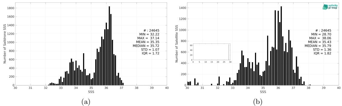
Figure 3: Histograms of SSS from Saildrone (a) and SMAP SSS L2 v5.0 (JPL) (b) considering all match-up pairs per bins of 0.1 over the Tropical Atlantic Ocean Pi-MEP region and for the full satellite product period.
