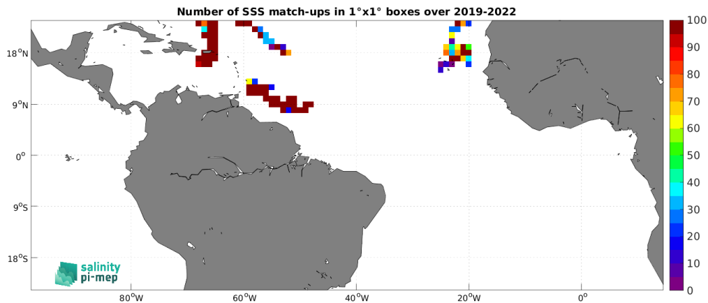
Figure 5: Number of SSS match-ups between Saildrone SSS and the SMAP SSS L2 v5.0 (JPL) SSS product for the Tropical Atlantic Ocean Pi-MEP region over 1^\circ \times 1^\circ boxes and for the full satellite product period.
