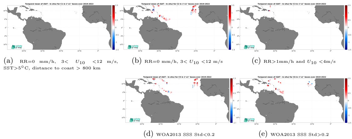
Figure 14: Temporal mean gridded over spatial boxes of size 1^\circ \times 1^\circ of \Delta\text{SSS} (SMAP SSS L2 v5.0 (JPL) - Saildrone) for 5 different subdatasets corresponding to:RR=0 mm/h, 3 < U_{10} < 12 m/s, SST>5°C, distance to coast > 800 km (a), RR=0 mm/h, 3 < U_{10} < 12 m/s (b), RR>1mm/h and U_{10} < 4 m/s (c), WOA2013 SSS Std<0.2 (d), WOA2013 SSS Std>0.2 (e).
