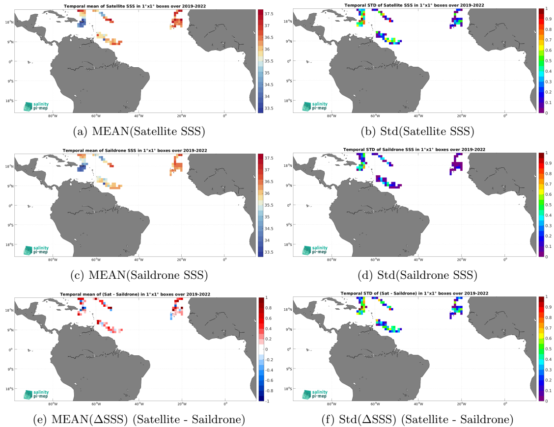
Figure 7: Temporal mean (left) and Std (right) of SSS from SMAP SSS L2 v5.0 (JPL) (top), Saildrone (middle), and of \Delta SSS (Satellite - Saildrone). Only match-up pairs are used to generate these maps.
