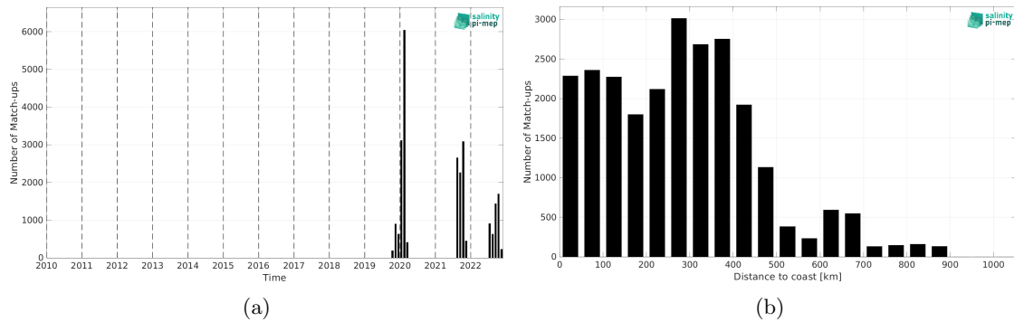
Figure 2: Number of match-ups between Saildrone and SMAP SSS L2 v5.0 (JPL) SSS as a function of time (a) and as function of the distance to coast (b) over the Tropical Atlantic Ocean Pi-MEP region and for the full satellite product period.
