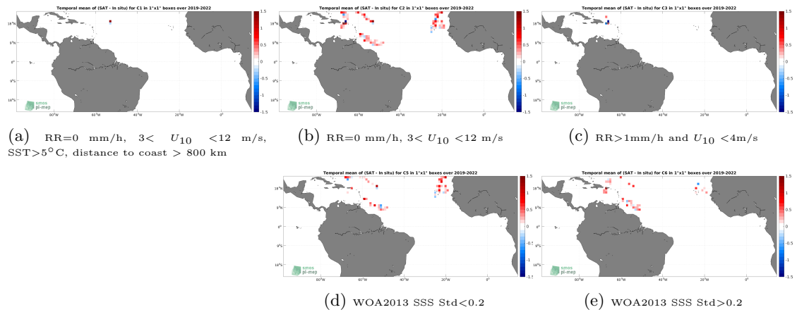
Figure 12: Temporal mean gridded over spatial boxes of size 1^\circ \times 1^\circ of \Delta SSS (SMAP SSS L2 v5.0 (JPL) - Saildrone) for 5 different subdatasets corresponding to:RR=0 mm/h, 3 < U_{10} < 12 m/s, SST >5^\circ\text{C} , distance to coast > 800 km (a), RR=0 mm/h, 3 < U_{10} < 12 m/s (b), RR >1 mm/h and U_{10} < 4 m/s (c), WOA2013 SSS Std <0.2 (d), WOA2013 SSS Std >0.2 (e).
