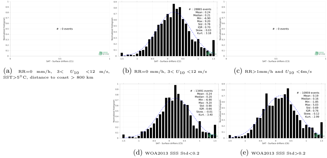
Figure 12: Normalized histogram of \Delta SSS (SMAP SSS L2 v5.0 (JPL) - Surface drifters) for 5 different subdatasets corresponding to: RR=0 mm/h, 3 < U_{10} < 12 m/s, SST > 5°C, distance to coast > 800 km (a), RR=0 mm/h, 3 < U_{10} < 12 m/s (b), RR > 1mm/h and U_{10} < 4 m/s (c), WOA2013 SSS Std < 0.2 (d), WOA2013 SSS Std > 0.2 (e).
