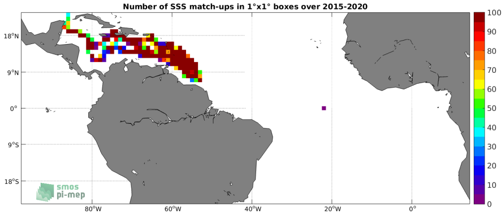
Figure 3: Number of SSS match-ups between Surface drifters SSS and the SMAP SSS L2 v5.0 (JPL) SSS product for the Tropical Atlantic Ocean Pi-MEP region over 1^\circ \times 1^\circ boxes and for the full satellite product period.
