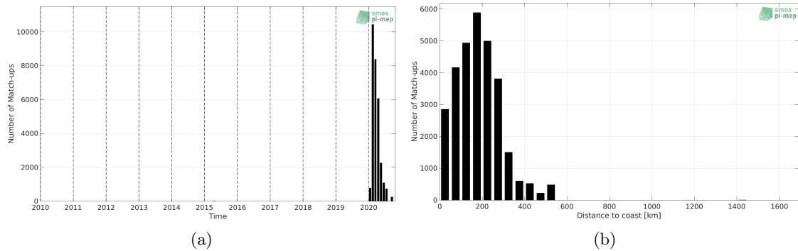
Figure 1: Number of match-ups between Surface drifters and SMAP SSS L2 v5.0 (JPL) SSS as a function of time (a) and as function of the distance to coast (b) over the Tropical Atlantic Ocean Pi-MEP region and for the full satellite product period.
