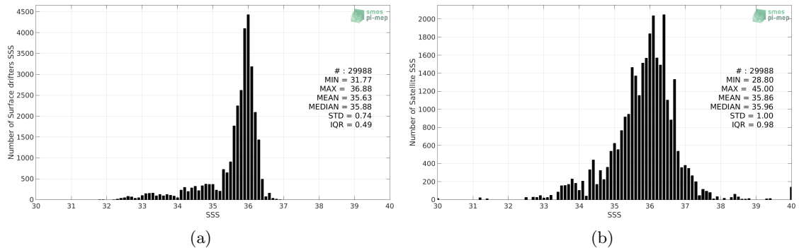
Figure 2: Histograms of SSS from Surface drifters (a) and SMAP SSS L2 v5.0 (JPL) (b) considering all match-up pairs per bins of 0.1 over the Tropical Atlantic Ocean Pi-MEP region and for the full satellite product period.
