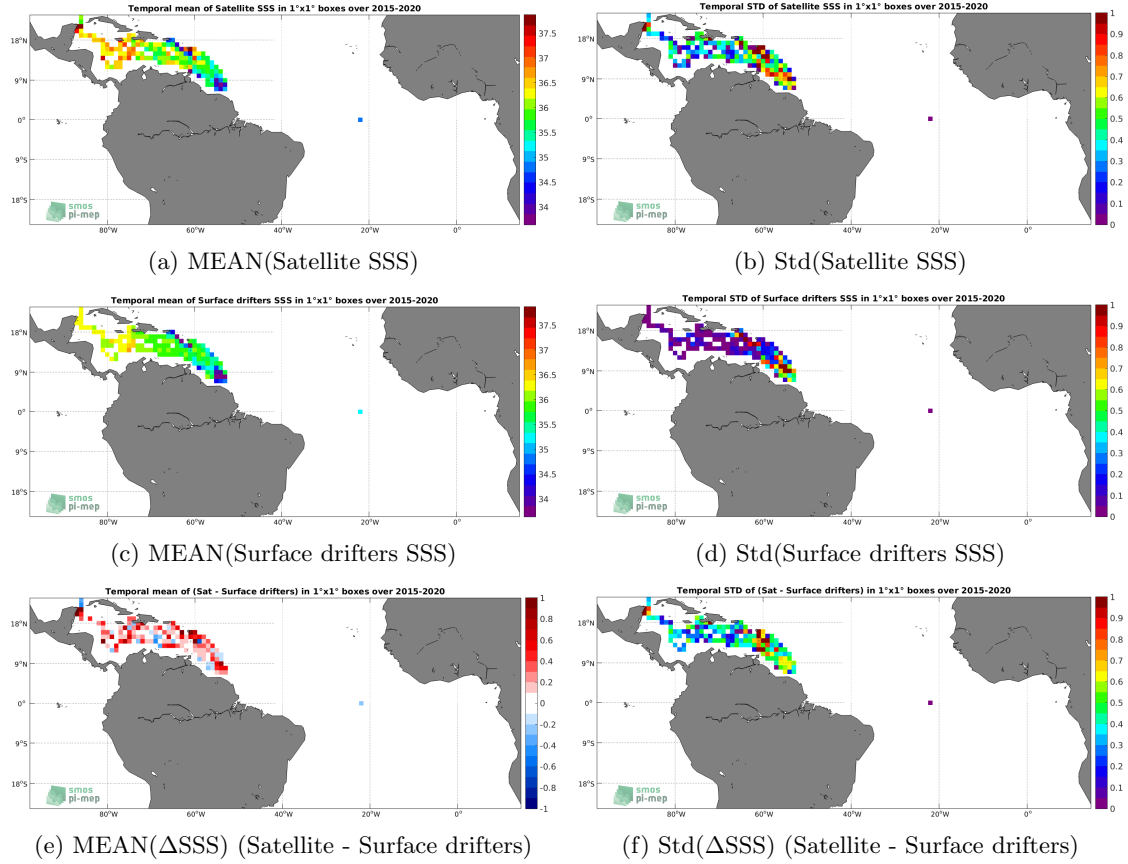
Figure 5: Temporal mean (left) and Std (right) of SSS from SMAP SSS L2 v5.0 (JPL) (top), Surface drifters (middle), and of \Delta SSS (Satellite - Surface drifters). Only match-up pairs are used to generate these maps.
