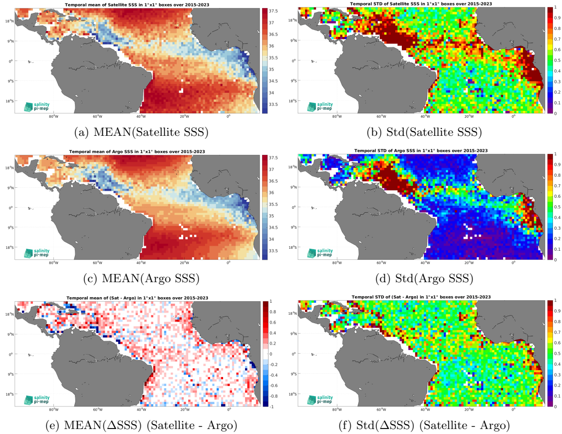
Figure 6: Temporal mean (left) and Std (right) of SSS from SMAP SSS L2 v5.0 (JPL) (top), Argo (middle), and of \Delta SSS (Satellite - Argo). Only match-up pairs are used to generate these maps.
