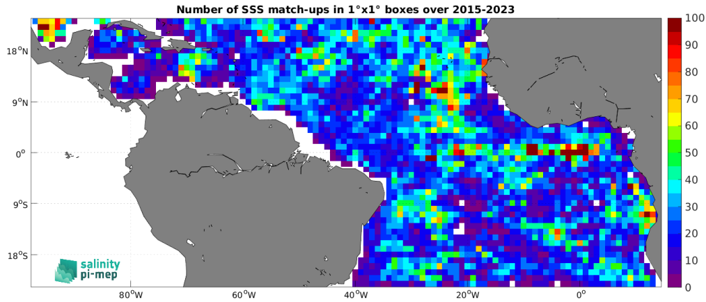
Figure 4: Number of SSS match-ups between Argo SSS and the SMAP SSS L2 v5.0 (JPL) SSS product for the Tropical Atlantic Ocean Pi-MEP region over 1^\circ \times 1^\circ boxes and for the full satellite product period.
