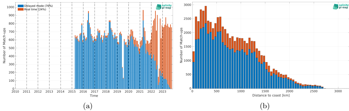
Figure 1: Number of match-ups between Argo and SMAP SSS L2 v5.0 (JPL) SSS as a function of time (a) and as function of the distance to coast (b) over the Tropical Atlantic Ocean Pi-MEP region and for the full satellite product period.
