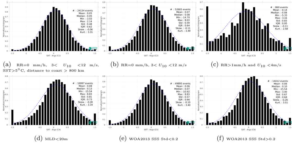
Figure 13: Normalized histogram of \Delta\text{SSS} (SMAP SSS L2 v5.0 (JPL) - Argo) for 6 different subdatasets corresponding to: RR=0 mm/h, 3 < U_{10} < 12 m/s, SST>5°C, distance to coast > 800 km (a), RR=0 mm/h, 3 < U_{10} < 12 m/s (b), RR>1mm/h and U_{10} < 4 m/s (c), MLD<20m (d), WOA2013 SSS Std<0.2 (e), WOA2013 SSS Std>0.2 (f).
