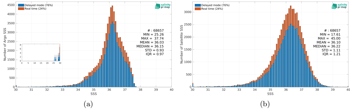
Figure 2: Histograms of SSS from Argo (a) and SMAP SSS L2 v5.0 (JPL) (b) considering all match-up pairs per bins of 0.1 over the Tropical Atlantic Ocean Pi-MEP region and for the full satellite product period.
