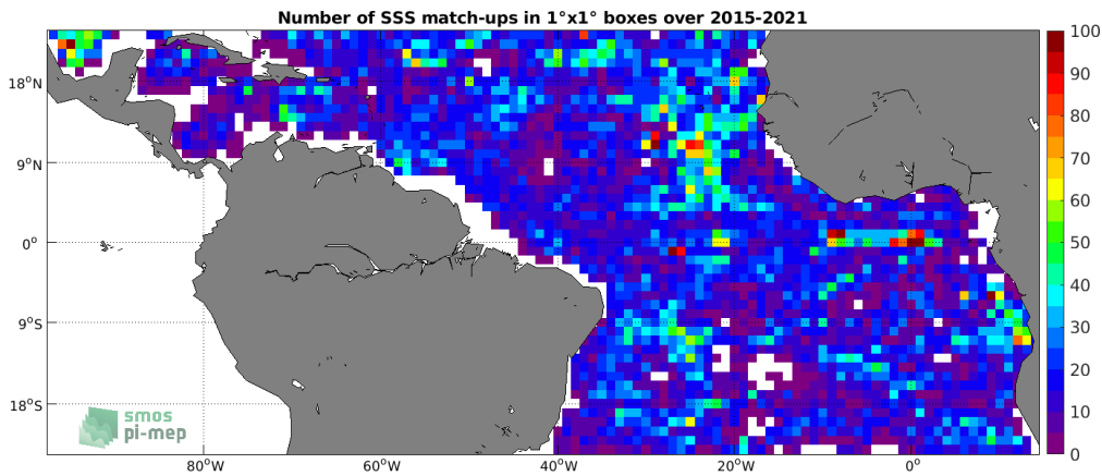
Figure 4: Number of SSS match-ups between Argo SSS and the SMAP SSS L2 v5.0 (JPL) SSS product for the Tropical Atlantic Ocean Pi-MEP region over 1°x1° boxes and for the full satellite product period.
