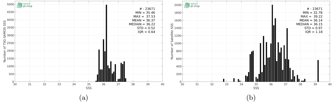
Figure 2: Histograms of SSS from TSG-SAMOS (a) and SMAP-L2-JPL-V4 (b) considering all match-up pairs per bins of 0.1 over the Tropical Atlantic Ocean Pi-MEP region and for the full satellite product period.
