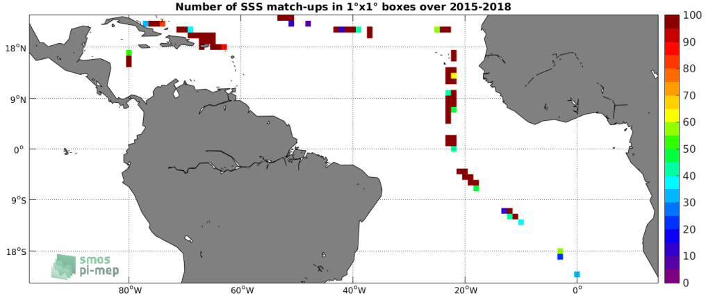
Figure 4: Number of SSS match-ups between TSG-SAMOS SSS and the SMAP-L2-JPL-V4 SSS product for the Tropical Atlantic Ocean Pi-MEP region over 1^\circ \times 1^\circ boxes and for the full satellite product period.
