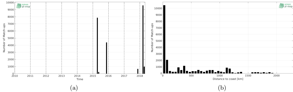
Figure 1: Number of match-ups between TSG-SAMOS and SMAP-L2-JPL-V4 SSS as a function of time (a) and as function of the distance to coast (b) over the Tropical Atlantic Ocean Pi-MEP region and for the full satellite product period.
