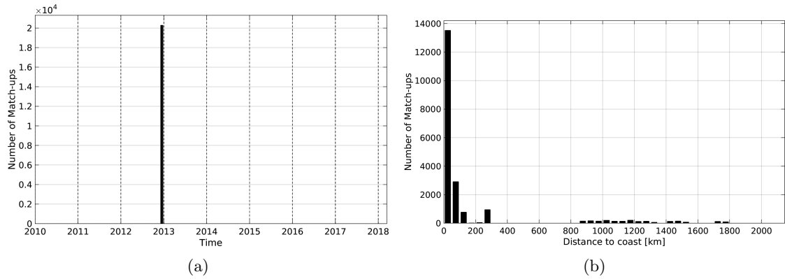
Figure 1: Number of match-ups between TSG-SAMOS and SMAP-L2-JPL-V4 SSS as a function of time (a) and as function of the distance to coast (b) over the Tropical Atlantic Ocean Pi-MEP region and for the full satellite product period.
