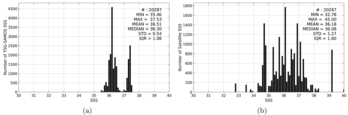
Figure 2: Histograms of SSS from TSG-SAMOS (a) and SMAP-L2-JPL-V4 (b) considering all match-up pairs per bins of 0.1 over the Tropical Atlantic Ocean Pi-MEP region and for the full satellite product period.
