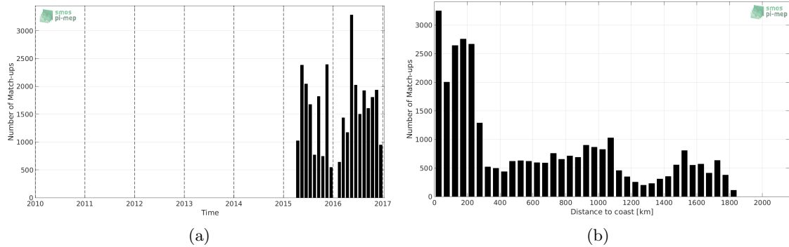
Figure 1: Number of match-ups between TSG-LEGOS-DM and SMAP-L2-JPL-V4 SSS as a function of time (a) and as function of the distance to coast (b) over the Tropical Atlantic Ocean Pi-MEP region and for the full satellite product period.
