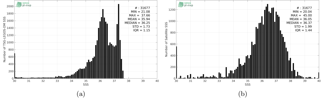
Figure 2: Histograms of SSS from TSG-LEGOS-DM (a) and SMAP-L2-JPL-V4 (b) considering all match-up pairs per bins of 0.1 over the Tropical Atlantic Ocean Pi-MEP region and for the full satellite product period.
