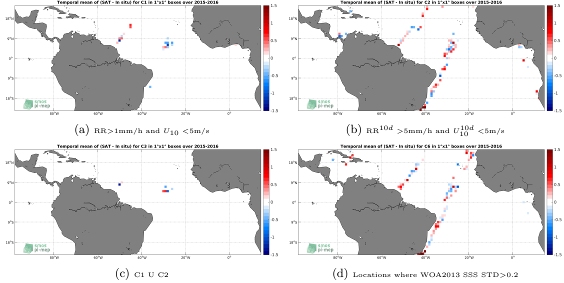
Figure 12: Temporal mean gridded over spatial boxes of size 1^\circ \times 1^\circ of \Delta SSS (SMAP-L2-JPL-V4 - TSG-LEGOS-DM) for 4 different subdatasets corresponding to: RR > 1\text{mm/h} and U_{10} < 5\text{m/s} (a), RR^{10d} > 5\text{mm/h} and U_{10}^{10d} < 5\text{m/s} (b), C1 U C2 (c), Locations where WOA2013 SSS STD > 0.2 (d).
