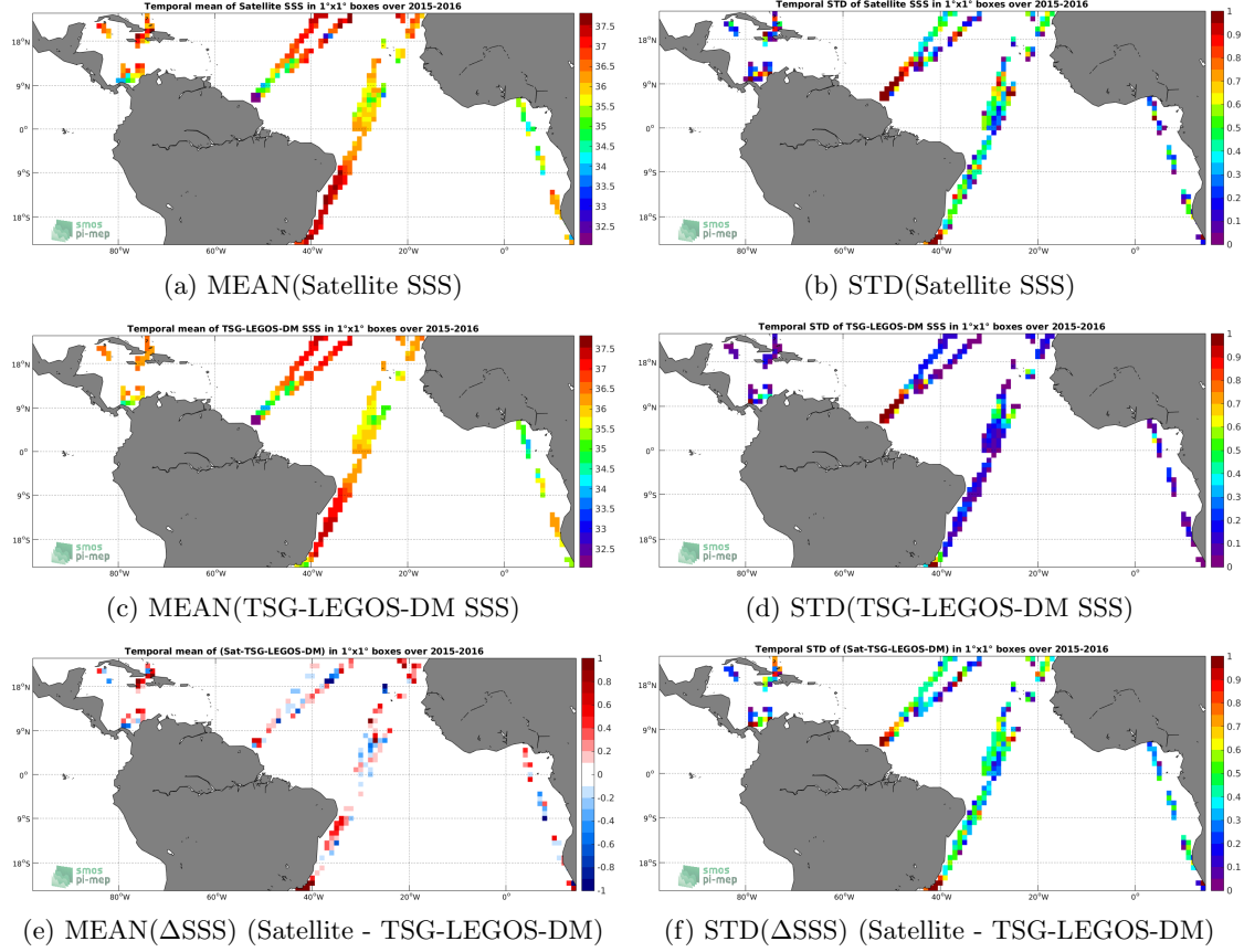
Figure 6: Temporal mean (left) and STD (right) of SSS from SMAP-L2-JPL-V4 (top), TSG-LEGOS-DM (middle), and of \Delta\text{SSS} (Satellite - TSG-LEGOS-DM). Only match-up pairs are used to generate these maps.
