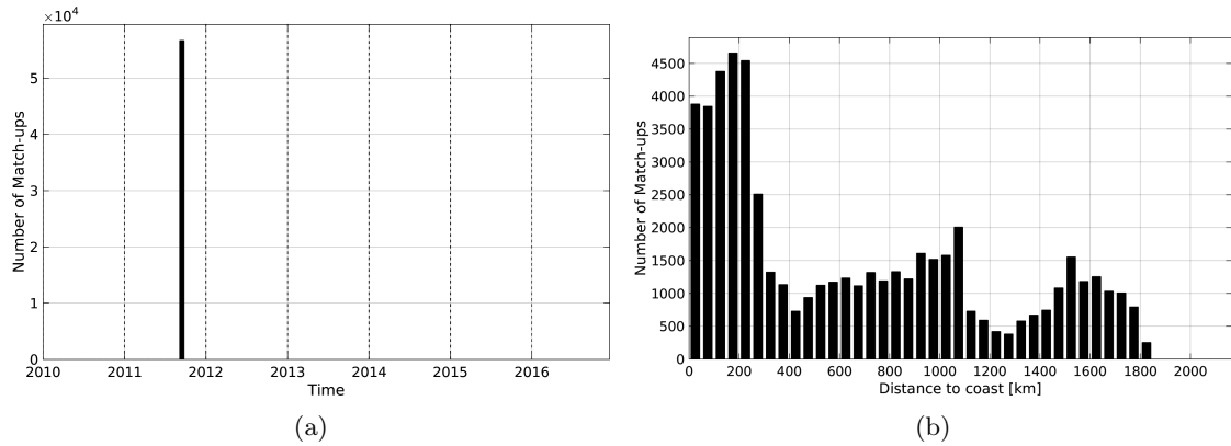
Figure 1: Number of match-ups between TSG-LEGOS-DM and SMAP-L2-JPL-V4 SSS as a function of time (a) and as function of the distance to coast (b) over the Tropical Atlantic Ocean Pi-MEP region and for the full satellite product period.
