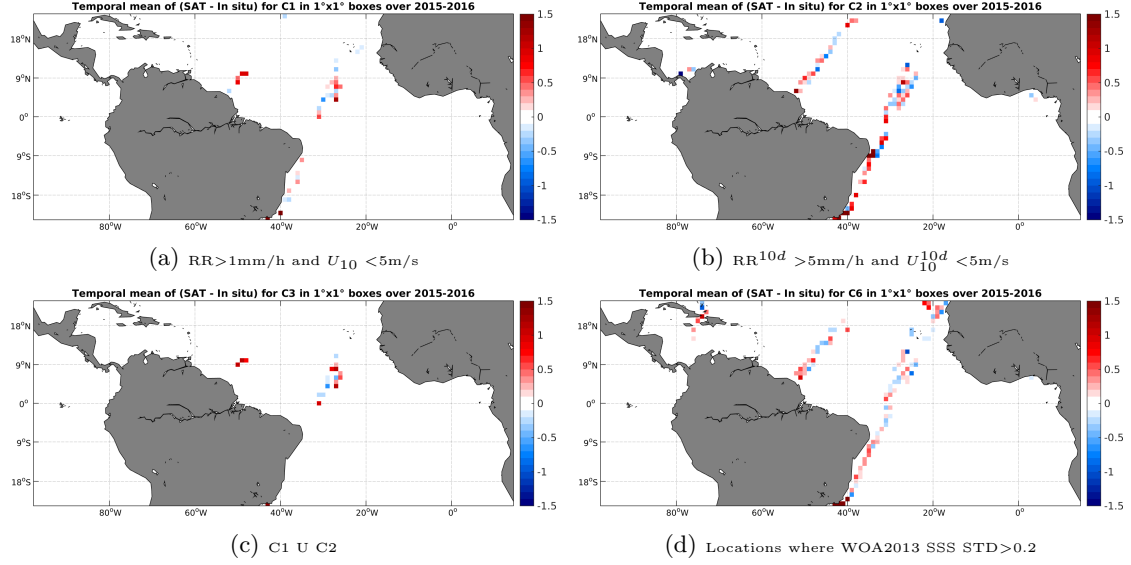
Figure 12: Temporal mean gridded over spatial boxes of size 1^\circ \times 1^\circ of \Delta SSS (SMAP-L2-JPL-V4 - TSG-LEGOS-DM) for 4 different subdatasets corresponding to: RR > 1 mm/h and U_{10} < 5 m/s (a), RR^{10d} > 5 mm/h and U_{10}^{10d} < 5 m/s (b), C1 U C2 (c), Locations where WOA2013 SSS STD > 0.2 (d).
