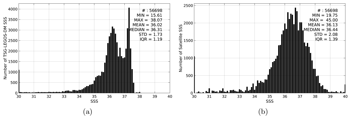
Figure 2: Histograms of SSS from TSG-LEGOS-DM (a) and SMAP-L2-JPL-V4 (b) considering all match-up pairs per bins of 0.1 over the Tropical Atlantic Ocean Pi-MEP region and for the full satellite product period.
