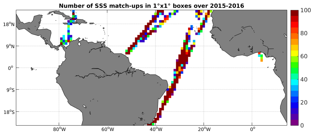
Figure 4: Number of SSS match-ups between TSG-LEGOS-DM SSS and the SMAP-L2-JPL-V4 SSS product for the Tropical Atlantic Ocean Pi-MEP region over 1°x1° boxes and for the full satellite product period.
