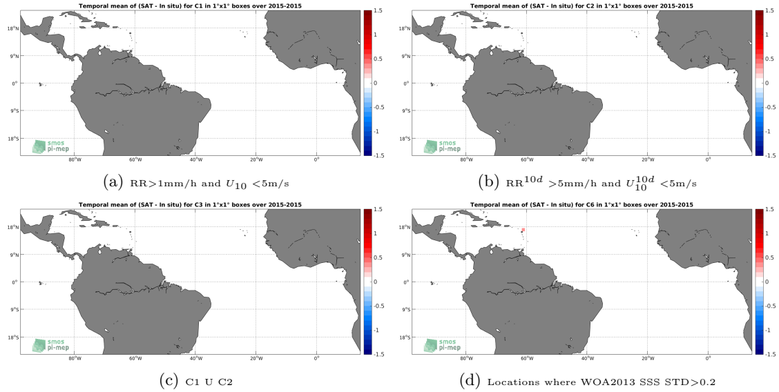
Figure 12: Temporal mean gridded over spatial boxes of size 1^\circ \times 1^\circ of \Delta SSS (SMAP-L2-JPL-V4 - TSG-GOSUD-Sailing-ship) for 4 different subdatasets corresponding to: RR > 1\text{mm/h} and U_{10} < 5\text{m/s} (a), RR^{10d} > 5\text{mm/h} and U_{10}^{10d} < 5\text{m/s} (b), C1 U C2 (c), Locations where WOA2013 SSS STD > 0.2 (d).
