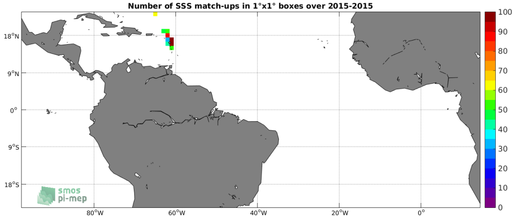
Figure 4: Number of SSS match-ups between TSG-GOSUD-Sailing-ship SSS and the SMAP-L2-JPL-V4 SSS product for the Tropical Atlantic Ocean Pi-MEP region over 1^\circ \times 1^\circ boxes and for the full satellite product period.
