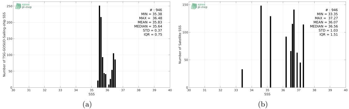
Figure 2: Histograms of SSS from TSG-GOSUD-Sailing-ship (a) and SMAP-L2-JPL-V4 (b) considering all match-up pairs per bins of 0.1 over the Tropical Atlantic Ocean Pi-MEP region and for the full satellite product period.
