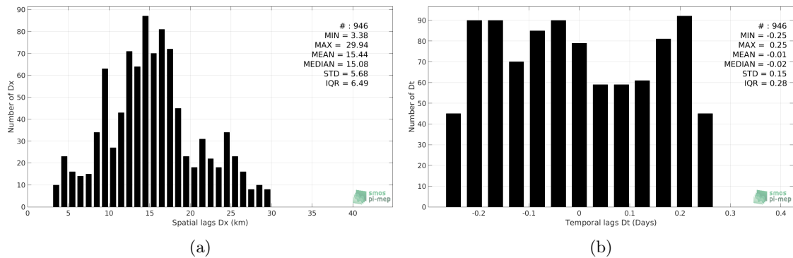
Figure 5: Histograms of the spatial (a) and temporal (b) lags between the time of the TSG-GOSUD-Sailing-ship measurements and the date of the corresponding SMAP-L2-JPL-V4 SSS product.
