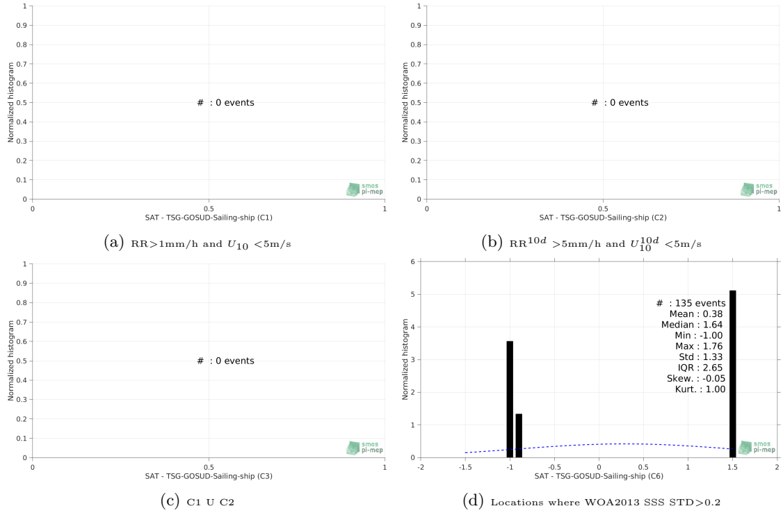
Figure 13: Normalized histogram of \Delta\text{SSS} (SMAP-L2-JPL-V4 - TSG-GOSUD-Sailing-ship) for 6 different subdatasets corresponding to: RR > 1\text{mm/h} and U_{10} < 5\text{m/s} (a), RR^{10d} > 5\text{mm/h} and U_{10}^{10d} < 5\text{m/s} (b), C1 U C2 (c), Locations where WOA2013 SSS STD > 0.2 (d).
