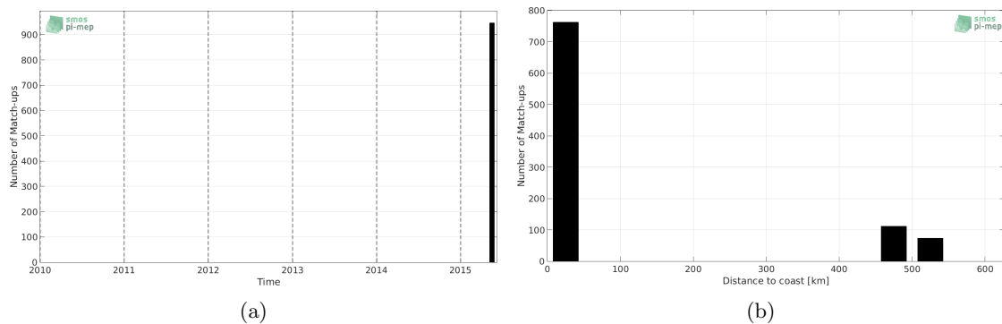
Figure 1: Number of match-ups between TSG-GOSUD-Sailing-ship and SMAP-L2-JPL-V4 SSS as a function of time (a) and as function of the distance to coast (b) over the Tropical Atlantic Ocean Pi-MEP region and for the full satellite product period.
