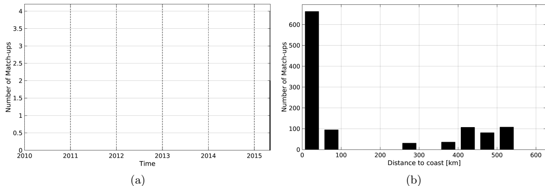
Figure 1: Number of match-ups between TSG-GOSUD-Sailing-ship and SMAP-L2-JPL-V4 SSS as a function of time (a) and as function of the distance to coast (b) over the Tropical Atlantic Ocean Pi-MEP region and for the full satellite product period.
