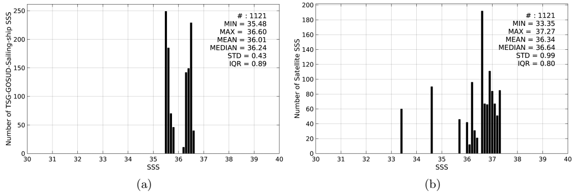
Figure 2: Histograms of SSS from TSG-GOSUD-Sailing-ship (a) and SMAP-L2-JPL-V4 (b) considering all match-up pairs per bins of 0.1 over the Tropical Atlantic Ocean Pi-MEP region and for the full satellite product period.
