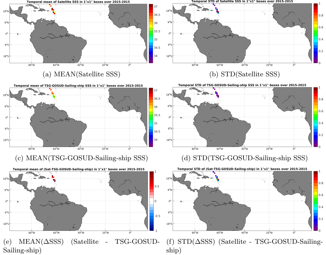
Figure 6: Temporal mean (left) and STD (right) of SSS from SMAP-L2-JPL-V4 (top), TSG-GOSUD-Sailing-ship (middle), and of \Delta\text{SSS} (Satellite - TSG-GOSUD-Sailing-ship). Only match-up pairs are used to generate these maps.
