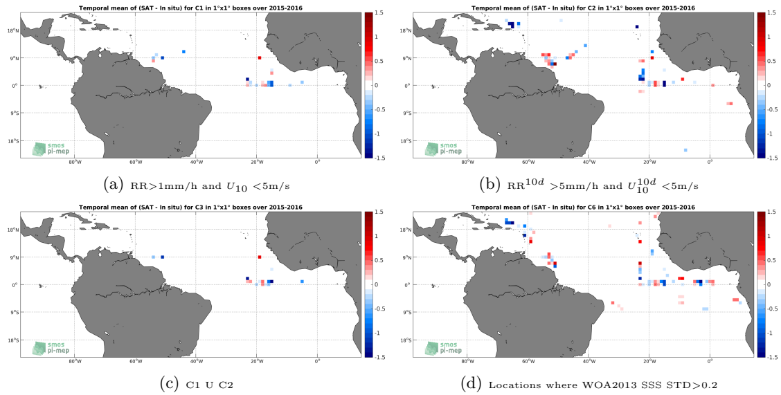
Figure 12: Temporal mean gridded over spatial boxes of size 1^\circ \times 1^\circ of \Delta SSS (SMAP-L2-JPL-V4 - TSG-GOSUD-Research-vessel) for 4 different subdatasets corresponding to:RR >1 mm/h and U_{10} < 5 m/s (a), RR 10d > 5 mm/h and U_{10}^{10d} < 5 m/s (b), C1 U C2 (c),Locations where WOA2013 SSS STD > 0.2 (d).
