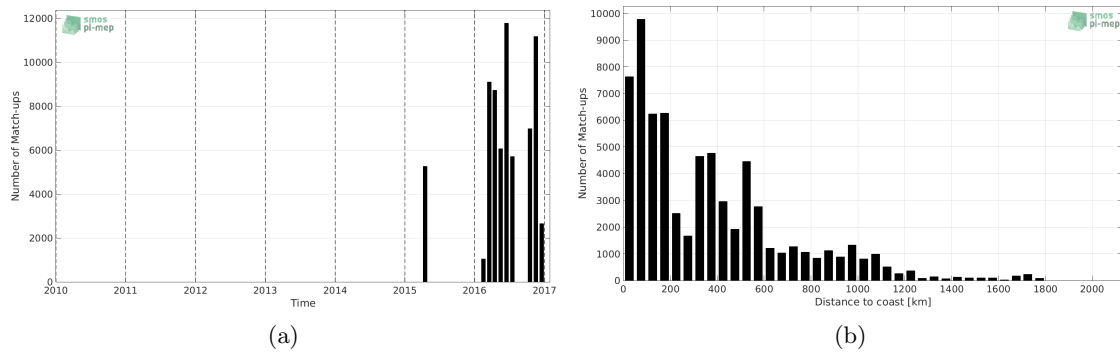
Figure 1: Number of match-ups between TSG-GOSUD-Research-vessel and SMAP-L2-JPL-V4 SSS as a function of time (a) and as function of the distance to coast (b) over the Tropical Atlantic Ocean Pi-MEP region and for the full satellite product period.
