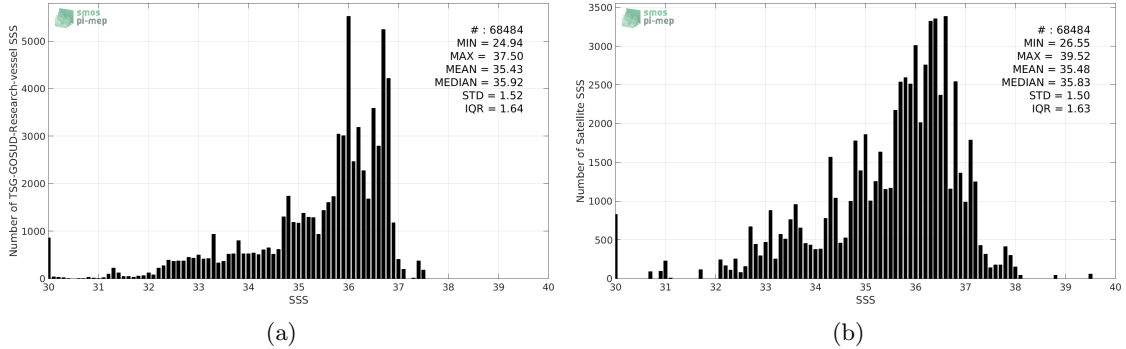
Figure 2: Histograms of SSS from TSG-GOSUD-Research-vessel (a) and SMAP-L2-JPL-V4 (b) considering all match-up pairs per bins of 0.1 over the Tropical Atlantic Ocean Pi-MEP region and for the full satellite product period.
