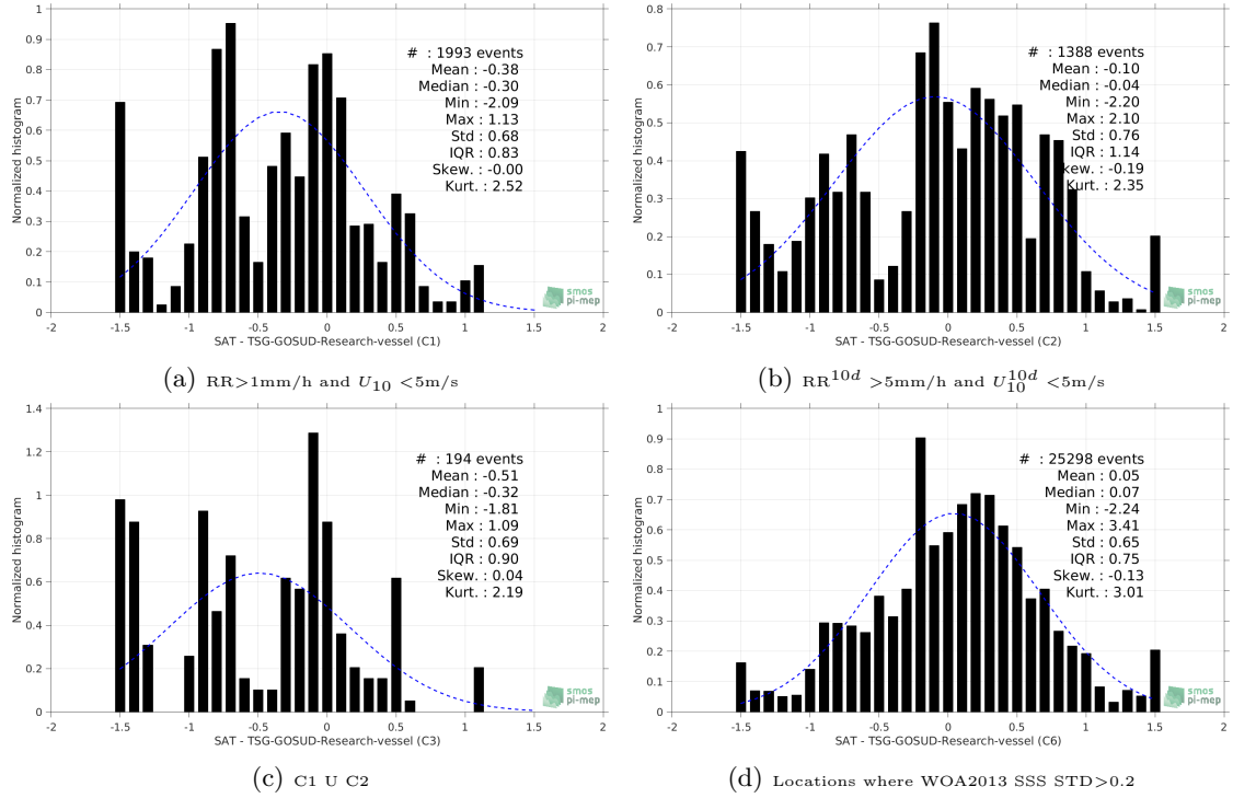
Figure 13: Normalized histogram of \Delta SSS (SMAP-L2-JPL-V4 - TSG-GOSUD-Research-vessel) for 6 different subdatasets corresponding to: RR > 1mm/h and U_{10} < 5 m/s (a), RR^{10d} > 5 mm/h and U_{10}^{10d} < 5 m/s (b), C1 U C2 (c), Locations where WOA2013 SSS STD > 0.2 (d).
