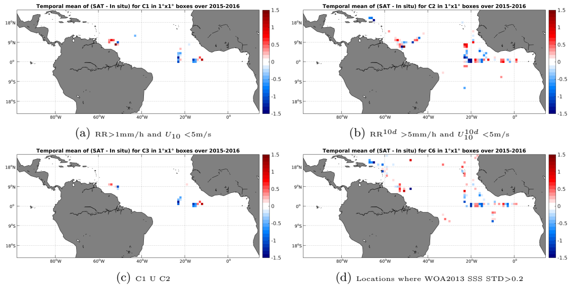
Figure 12: Temporal mean gridded over spatial boxes of size 1^\circ \times 1^\circ of \Delta SSS (SMAP-L2-JPL-V4 - TSG-GOSUD-Research-vessel) for 4 different subdatasets corresponding to: RR > 1\text{mm/h} and U_{10} < 5\text{m/s} (a), RR^{10d} > 5\text{mm/h} and U_{10}^{10d} < 5\text{m/s} (b), C1 U C2 (c), Locations where WOA2013 SSS STD > 0.2 (d).
