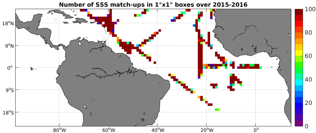
Figure 4: Number of SSS match-ups between TSG-GOSUD-Research-vessel SSS and the SMAP-L2-JPL-V4 SSS product for the Tropical Atlantic Ocean Pi-MEP region over 1^\circ \times 1^\circ boxes and for the full satellite product period.
