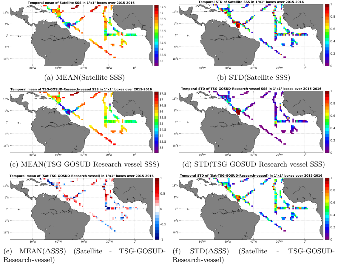
Figure 6: Temporal mean (left) and STD (right) of SSS from SMAP-L2-JPL-V4 (top), TSG-GOSUD-Research-vessel (middle), and of \Delta SSS (Satellite - TSG-GOSUD-Research-vessel). Only match-up pairs are used to generate these maps.
