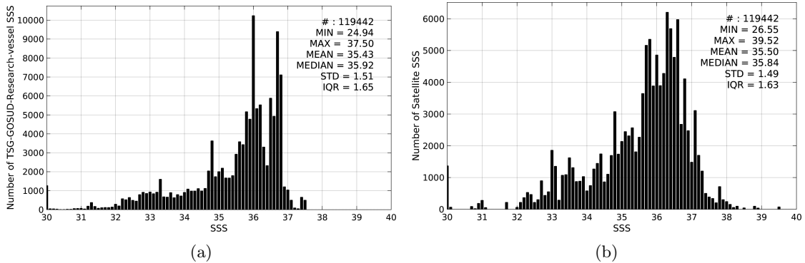
Figure 2: Histograms of SSS from TSG-GOSUD-Research-vessel (a) and SMAP-L2-JPL-V4 (b) considering all match-up pairs per bins of 0.1 over the Tropical Atlantic Ocean Pi-MEP region and for the full satellite product period.
