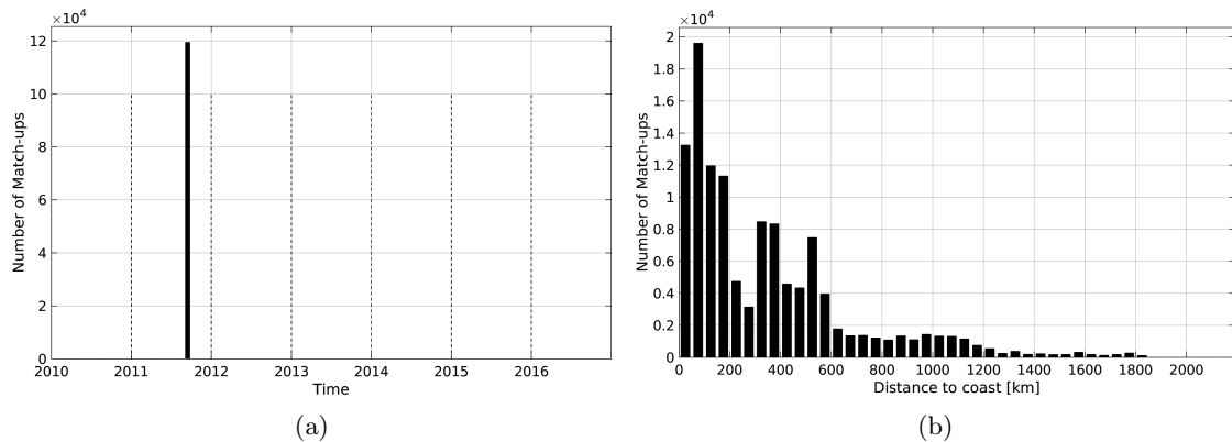
Figure 1: Number of match-ups between TSG-GOSUD-Research-vessel and SMAP-L2-JPL-V4 SSS as a function of time (a) and as function of the distance to coast (b) over the Tropical Atlantic Ocean Pi-MEP region and for the full satellite product period.
