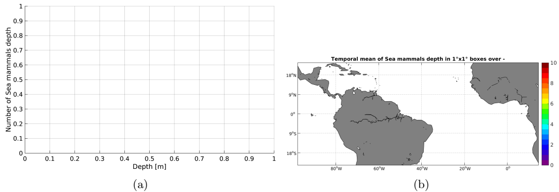
Figure 3: Histograms of the depth of the upper level SSS measurements from Sea mammals in the Match-up DataBase for the Tropical Atlantic Ocean Pi-MEP region (a) and temporal mean spatial distribution of pressure of the in situ SSS data over 1^\circ \times 1^\circ boxes and for the full satellite product period (b).
