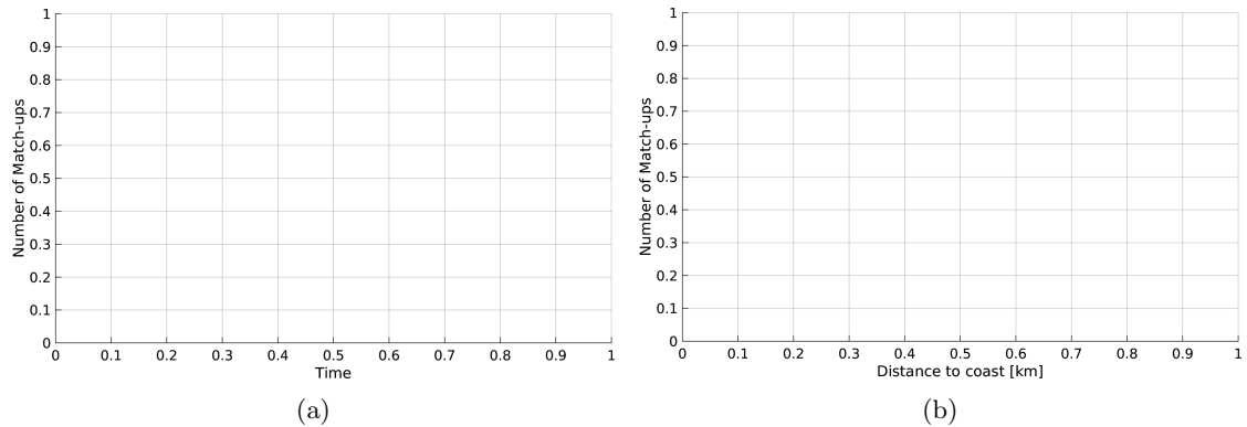
Figure 1: Number of match-ups between Sea mammals and SMAP-L2-JPL-V4 SSS as a function of time (a) and as function of the distance to coast (b) over the Tropical Atlantic Ocean Pi-MEP region and for the full satellite product period.
