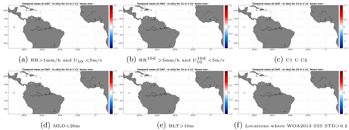
Figure 12: Temporal mean gridded over spatial boxes of size 1^\circ \times 1^\circ of \Delta SSS (SMAP-L2-JPL-V4 - Sea mammals) for 6 different subdatasets corresponding to: RR > 1 mm/h and U_{10} < 5 m/s (a), RR^{10d} > 5 mm/h and U_{10}^{10d} < 5 m/s (b), C1 U C2 (c), MLD < 20 m (d), BLT > 10 m (e), Locations where WOA2013 SSS STD > 0.2 (f).
