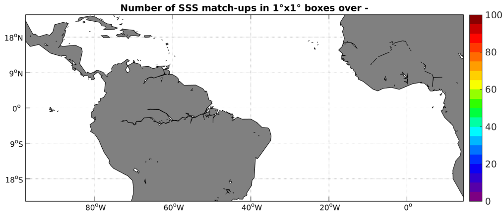
Figure 4: Number of SSS match-ups between Sea mammals SSS and the SMAP-L2-JPL-V4 SSS product for the Tropical Atlantic Ocean Pi-MEP region over 1^\circ \times 1^\circ boxes and for the full satellite product period.
