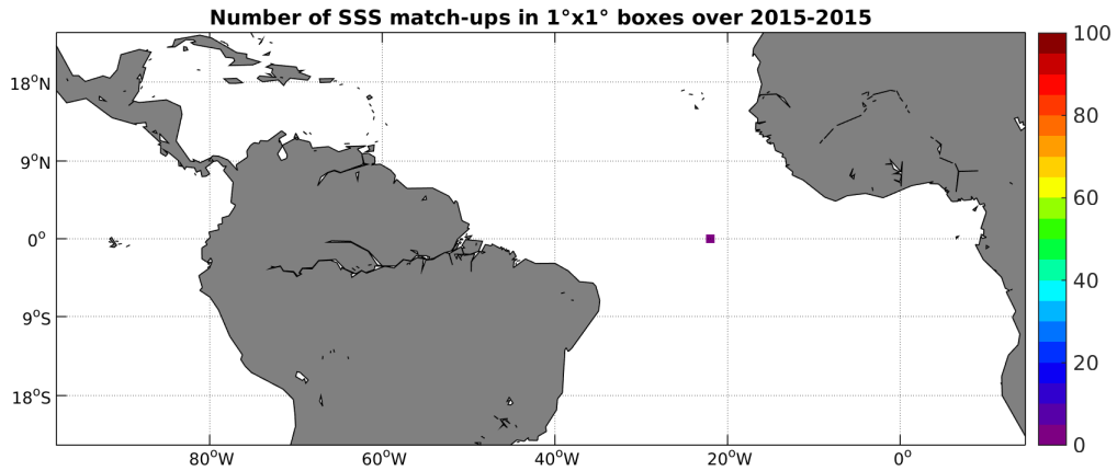
Figure 3: Number of SSS match-ups between Surface drifters SSS and the SMAP-L2-JPL-V4 SSS product for the Tropical Atlantic Ocean Pi-MEP region over 1°x1° boxes and for the full satellite product period.
