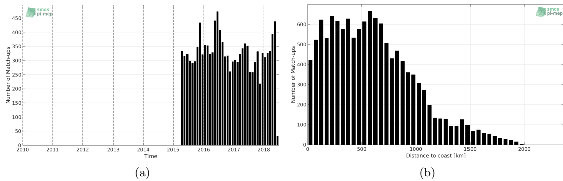
Figure 1: Number of match-ups between Argo and SMAP-L2-JPL-V4 SSS as a function of time (a) and as function of the distance to coast (b) over the Tropical Atlantic Ocean Pi-MEP region and for the full satellite product period.
