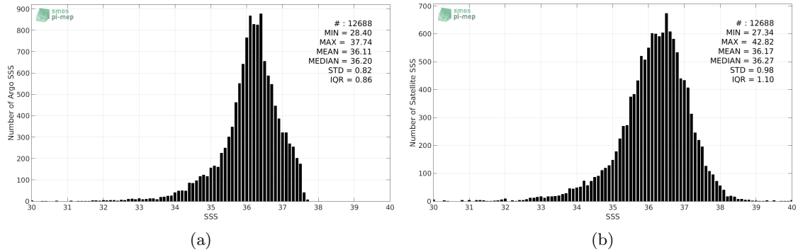
Figure 2: Histograms of SSS from Argo (a) and SMAP-L2-JPL-V4 (b) considering all match-up pairs per bins of 0.1 over the Tropical Atlantic Ocean Pi-MEP region and for the full satellite product period.
