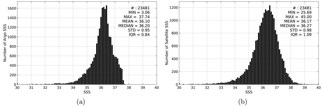
Figure 2: Histograms of SSS from Argo (a) and SMAP-L2-JPL-V4 (b) considering all match-up pairs per bins of 0.1 over the Tropical Atlantic Ocean Pi-MEP region and for the full satellite product period.
