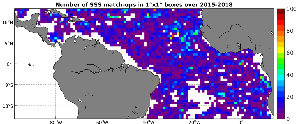
Figure 4: Number of SSS match-ups between Argo SSS and the SMAP-L2-JPL-V4 SSS product for the Tropical Atlantic Ocean Pi-MEP region over 1^\circ \times 1^\circ boxes and for the full satellite product period.
