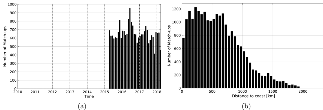
Figure 1: Number of match-ups between Argo and SMAP-L2-JPL-V4 SSS as a function of time (a) and as function of the distance to coast (b) over the Tropical Atlantic Ocean Pi-MEP region and for the full satellite product period.
