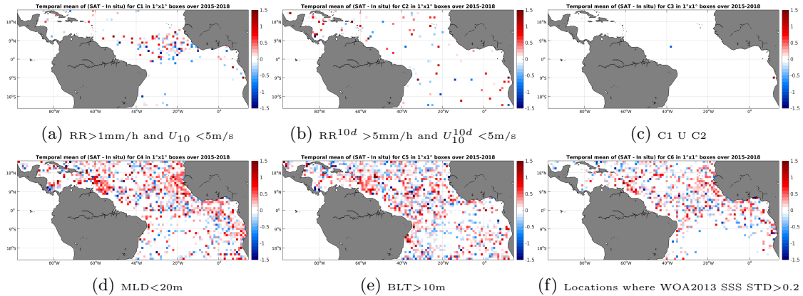
Figure 12: Temporal mean gridded over spatial boxes of size 1^\circ \times 1^\circ of \Delta SSS (SMAP-L2-JPL-V4 - Argo) for 6 different subdatasets corresponding to: RR > 1\text{mm/h} and U_{10} < 5\text{m/s} (a), RR^{10d} > 5\text{mm/h} and U_{10}^{10d} < 5\text{m/s} (b), C1 U C2 (c), MLD < 20\text{m} (d), BLT > 10\text{m} (e), Locations where WOA2013 SSS STD > 0.2 (f).
