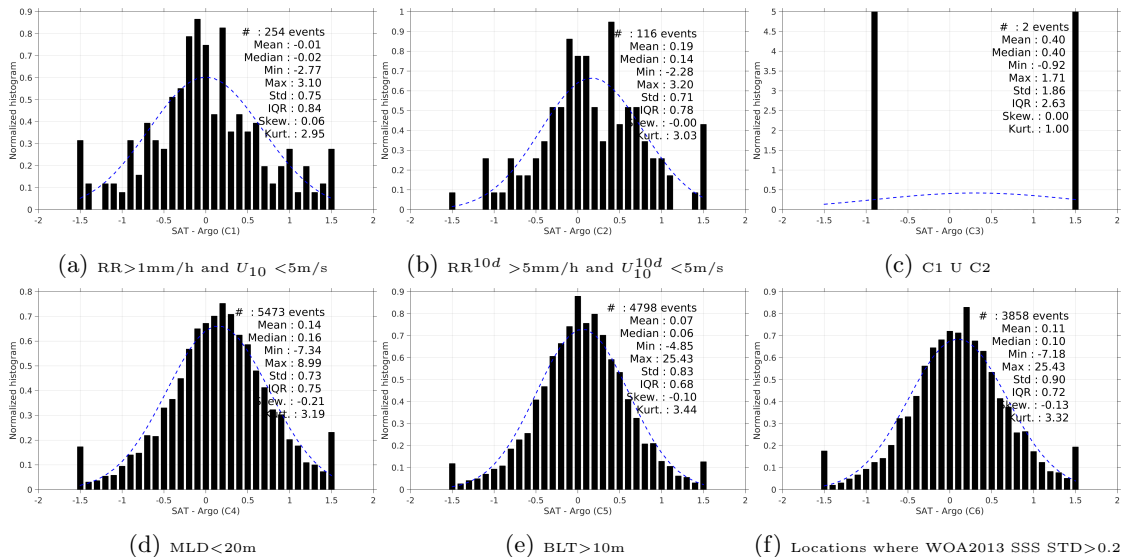
Figure 13: Normalized histogram of \Delta SSS (SMAP-L2-JPL-V4 - Argo) for 6 different subdatasets corresponding to: RR > 1\text{mm/h} and U_{10} < 5\text{m/s} (a), RR^{10d} > 5\text{mm/h} and U_{10}^{10d} < 5\text{m/s} (b), C1 U C2 (c), MLD < 20\text{m} (d), BLT > 10\text{m} (e), Locations where WOA2013 SSS STD > 0.2 (f).
