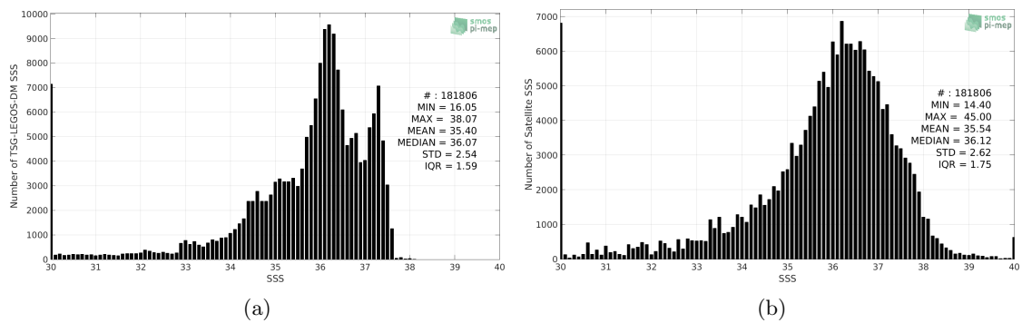
Figure 2: Histograms of SSS from TSG-LEGOS-DM (a) and SMAP-L2-JPL-V4.3 (b) considering all match-up pairs per bins of 0.1 over the Tropical Atlantic Ocean Pi-MEP region and for the full satellite product period.
