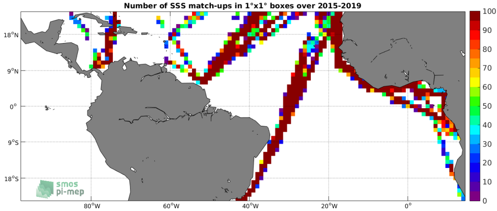
Figure 4: Number of SSS match-ups between TSG-LEGOS-DM SSS and the SMAP-L2-JPL-V4.3 SSS product for the Tropical Atlantic Ocean Pi-MEP region over 1^\circ \times 1^\circ boxes and for the full satellite product period.
