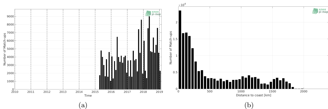
Figure 1: Number of match-ups between TSG-LEGOS-DM and SMAP-L2-JPL-V4.3 SSS as a function of time (a) and as function of the distance to coast (b) over the Tropical Atlantic Ocean Pi-MEP region and for the full satellite product period.
