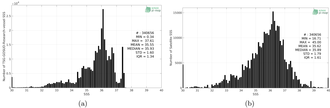
Figure 2: Histograms of SSS from TSG-GOSUD-Research-vessel (a) and SMAP-L2-JPL-V4.3 (b) considering all match-up pairs per bins of 0.1 over the Tropical Atlantic Ocean Pi-MEP region and for the full satellite product period.
