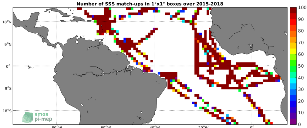
Figure 4: Number of SSS match-ups between TSG-GOSUD-Research-vessel SSS and the SMAP-L2-JPL-V4.3 SSS product for the Tropical Atlantic Ocean Pi-MEP region over 1^\circ \times 1^\circ boxes and for the full satellite product period.
