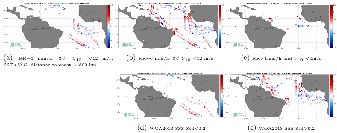
Figure 12: Temporal mean gridded over spatial boxes of size 1^\circ \times 1^\circ of \Delta SSS (SMAP-L2-JPL-V4.3 - TSG-GOSUD-Research-vessel) for 5 different subdatasets corresponding to: RR=0 mm/h, 3 < U_{10} < 12 m/s, SST > 5°C, distance to coast > 800 km (a), RR=0 mm/h, 3 < U_{10} < 12 m/s (b), RR > 1mm/h and U_{10} < 4 m/s (c), WOA2013 SSS Std < 0.2 (d), WOA2013 SSS Std > 0.2 (e).
