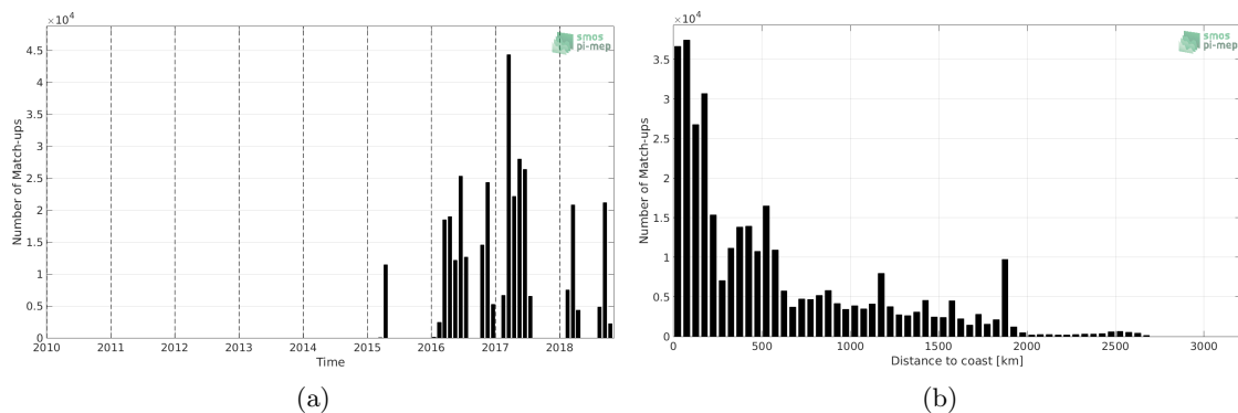
Figure 1: Number of match-ups between TSG-GOSUD-Research-vessel and SMAP-L2-JPL-V4.3 SSS as a function of time (a) and as function of the distance to coast (b) over the Tropical Atlantic Ocean Pi-MEP region and for the full satellite product period.
