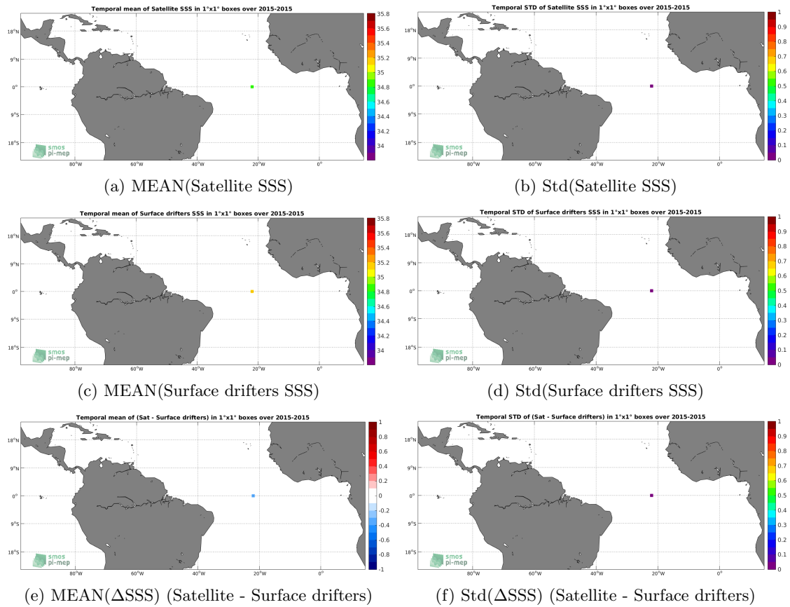
Figure 5: Temporal mean (left) and Std (right) of SSS from SMAP-L2-JPL-V4.3 (top), Surface drifters (middle), and of \Delta SSS (Satellite - Surface drifters). Only match-up pairs are used to generate these maps.
