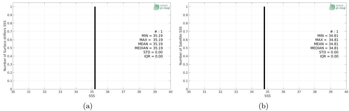
Figure 2: Histograms of SSS from Surface drifters (a) and SMAP-L2-JPL-V4.3 (b) considering all match-up pairs per bins of 0.1 over the Tropical Atlantic Ocean Pi-MEP region and for the full satellite product period.
