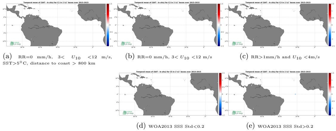
Figure 11: Temporal mean gridded over spatial boxes of size 1^{\circ}\times 1^{\circ} of \Delta\text{SSS} (SMAP-L2-JPL-V4.3 - Surface drifters) for 5 different subdatasets corresponding to:RR=0 mm/h, 3 < U_{10} < 12 m/s, SST >5^{\circ}\text{C} , distance to coast > 800 km (a), RR=0 mm/h, 3 < U_{10} < 12 m/s (b), RR >1 mm/h and U_{10} < 4 m/s (c), WOA2013 SSS Std <0.2 (d), WOA2013 SSS Std >0.2 (e).
