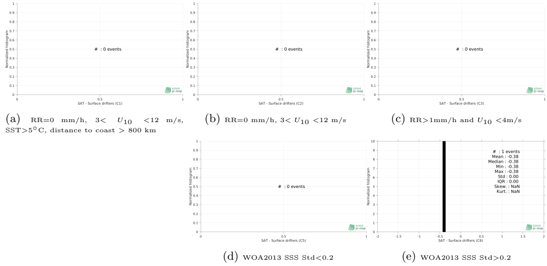
Figure 12: Normalized histogram of \Delta\text{SSS} (SMAP-L2-JPL-V4.3 - Surface drifters) for 5 different subdatasets corresponding to: RR=0 mm/h, 3 < U_{10} < 12 m/s, SST > 5^\circ\text{C} , distance to coast > 800 km (a), RR=0 mm/h, 3 < U_{10} < 12 m/s (b), RR > 1\text{mm/h} and U_{10} < 4\text{m/s} (c), WOA2013 SSS Std < 0.2 (d), WOA2013 SSS Std > 0.2 (e).
