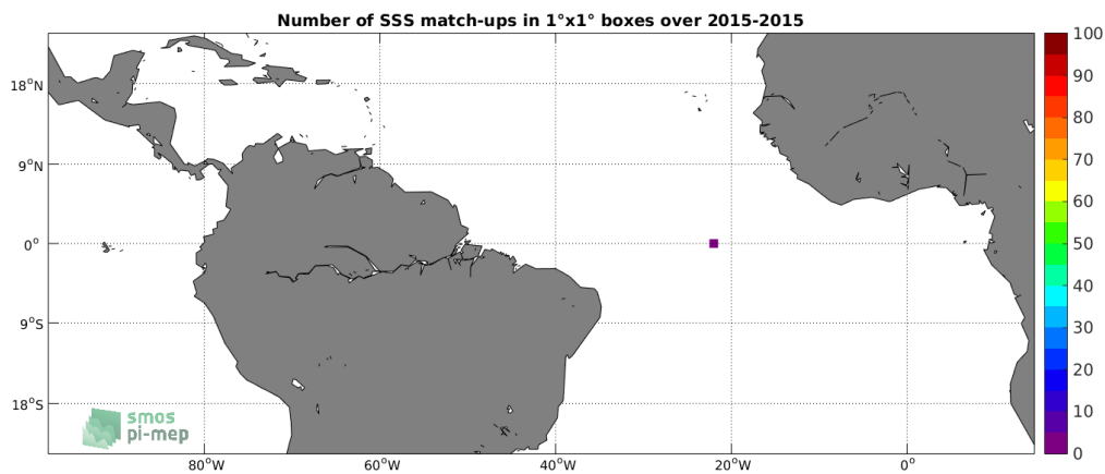
Figure 3: Number of SSS match-ups between Surface drifters SSS and the SMAP-L2-JPL-V4.3 SSS product for the Tropical Atlantic Ocean Pi-MEP region over 1^\circ \times 1^\circ boxes and for the full satellite product period.
