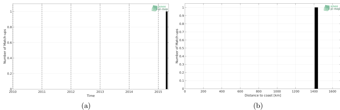
Figure 1: Number of match-ups between Surface drifters and SMAP-L2-JPL-V4.3 SSS as a function of time (a) and as function of the distance to coast (b) over the Tropical Atlantic Ocean Pi-MEP region and for the full satellite product period.
