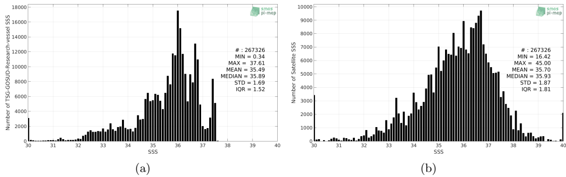
Figure 2: Histograms of SSS from TSG-GOSUD-Research-vessel (a) and SMAP-L2-JPL-V4.2 (b) considering all match-up pairs per bins of 0.1 over the Tropical Atlantic Ocean Pi-MEP region and for the full satellite product period.
