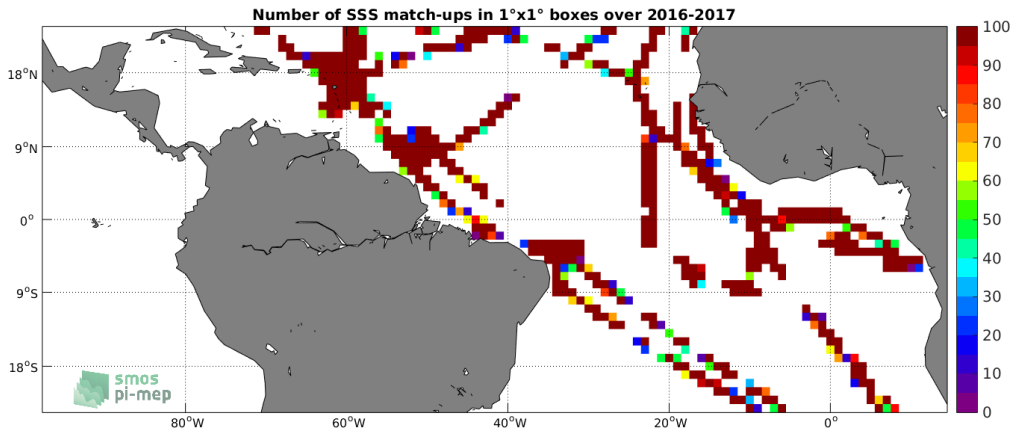
Figure 4: Number of SSS match-ups between TSG-GOSUD-Research-vessel SSS and the SMAP-L2-JPL-V4.2 SSS product for the Tropical Atlantic Ocean Pi-MEP region over 1^\circ \times 1^\circ boxes and for the full satellite product period.
