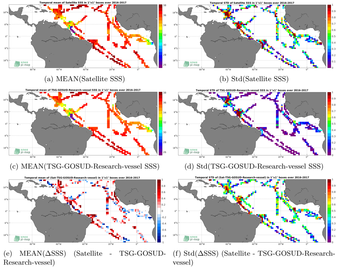
Figure 6: Temporal mean (left) and Std (right) of SSS from SMAP-L2-JPL-V4.2 (top), TSG-GOSUD-Research-vessel (middle), and of \Delta SSS (Satellite - TSG-GOSUD-Research-vessel). Only match-up pairs are used to generate these maps.
