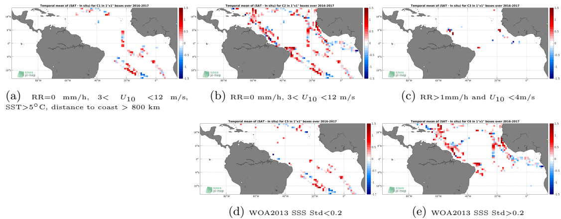
Figure 12: Temporal mean gridded over spatial boxes of size 1^\circ \times 1^\circ of \Delta SSS (SMAP-L2-JPL-V4.2 - TSG-GOSUD-Research-vessel) for 5 different subdatasets corresponding to:RR=0 mm/h, 3 < U_{10} < 12 m/s, SST >5^\circ\text{C} , distance to coast > 800 km (a), RR=0 mm/h, 3 < U_{10} < 12 m/s (b), RR >1 mm/h and U_{10} < 4 m/s (c), WOA2013 SSS Std <0.2 (d), WOA2013 SSS Std >0.2 (e).
