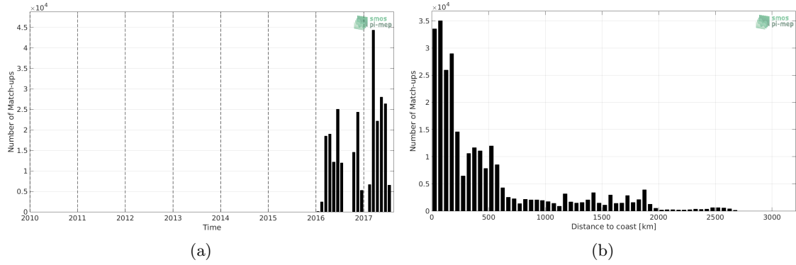
Figure 1: Number of match-ups between TSG-GOSUD-Research-vessel and SMAP-L2-JPL-V4.2 SSS as a function of time (a) and as function of the distance to coast (b) over the Tropical Atlantic Ocean Pi-MEP region and for the full satellite product period.
