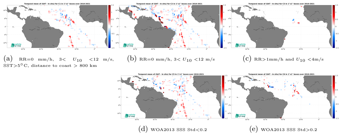
Figure 14: Temporal mean gridded over spatial boxes of size 1^\circ \times 1^\circ of \Delta SSS (ISAS v7 - Monthly (Ifremer-LOPS-CMEMS) - TSG (GOSUD-Sailing-ship)) for 5 different subdatasets corresponding to:RR=0 mm/h, 3 < U_{10} < 12 m/s, SST>5°C, distance to coast > 800 km (a), RR=0 mm/h, 3 < U_{10} < 12 m/s (b), RR>1mm/h and U_{10} < 4 m/s (c), WOA2013 SSS Std<0.2 (d), WOA2013 SSS Std>0.2 (e).
