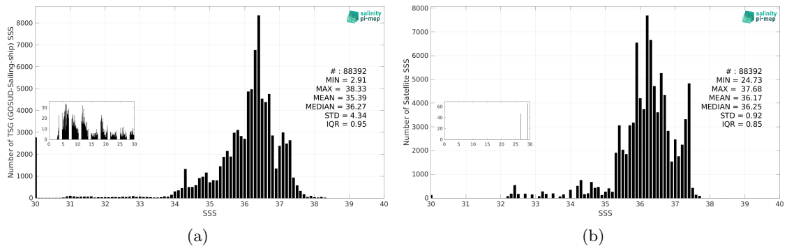
Figure 3: Histograms of SSS from TSG (GOSUD-Sailing-ship) (a) and ISAS v7 - Monthly (Ifremer-LOPS-CMEMS) (b) considering all match-up pairs per bins of 0.1 over the Tropical Atlantic Ocean Pi-MEP region and for the full satellite product period.
