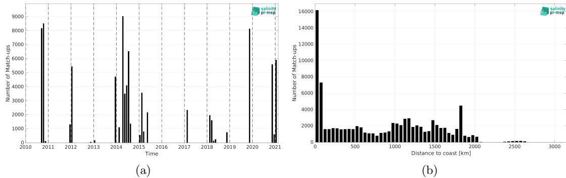
Figure 2: Number of match-ups between TSG (GOSUD-Sailing-ship) and ISAS v7 - Monthly (Ifremer-LOPS-CMEMS) SSS as a function of time (a) and as function of the distance to coast (b) over the Tropical Atlantic Ocean Pi-MEP region and for the full satellite product period.
