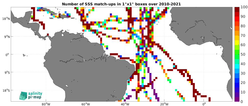
Figure 5: Number of SSS match-ups between TSG (GOSUD-Sailing-ship) SSS and the ISAS v7 - Monthly (Ifremer-LOPS-CMEMS) SSS product for the Tropical Atlantic Ocean Pi-MEP region over 1^\circ \times 1^\circ boxes and for the full satellite product period.
