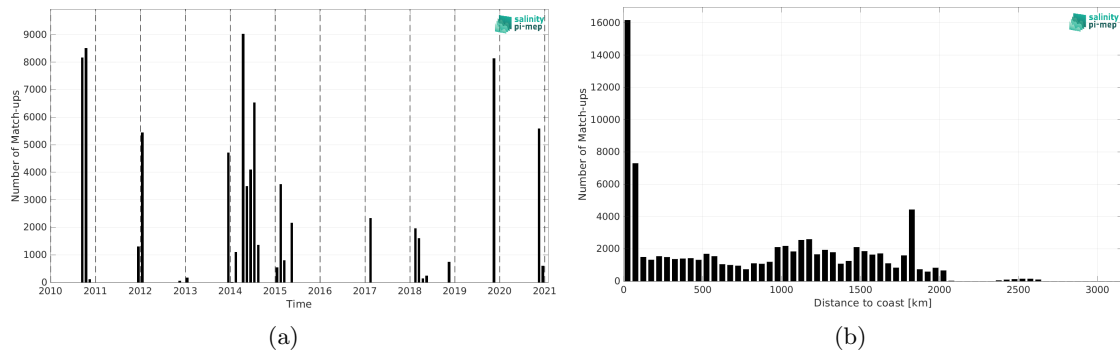
Figure 2: Number of match-ups between TSG (GOSUD-Sailing-ship) and ISAS SSS as a function of time (a) and as function of the distance to coast (b) over the Tropical Atlantic Ocean Pi-MEP region and for the full satellite product period.
