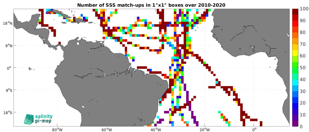
Figure 5: Number of SSS match-ups between TSG (GOSUD-Sailing-ship) SSS and the ISAS SSS product for the Tropical Atlantic Ocean Pi-MEP region over 1^\circ \times 1^\circ boxes and for the full satellite product period.
