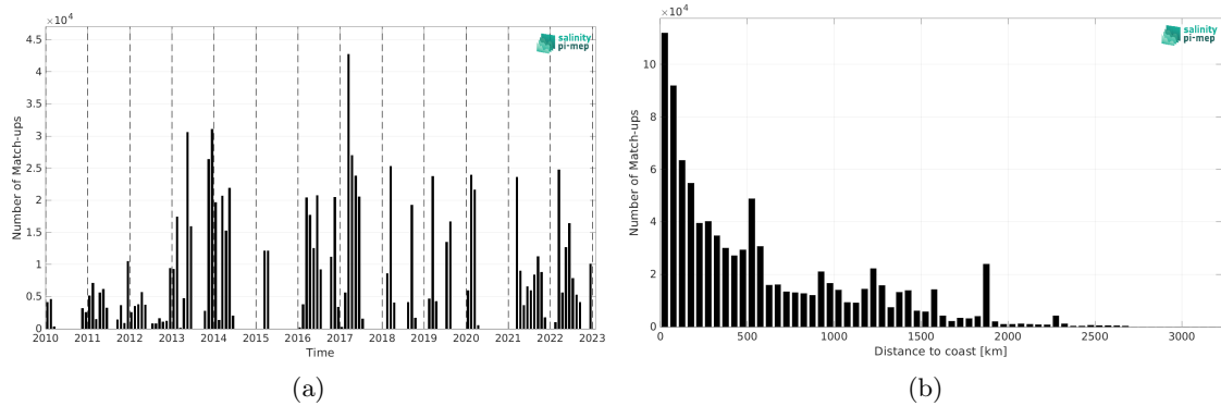
Figure 2: Number of match-ups between TSG (GOSUD-Research-vessel) and ISAS v7 - Monthly (Ifremer-LOPS-CMEMS) SSS as a function of time (a) and as function of the distance to coast (b) over the Tropical Atlantic Ocean Pi-MEP region and for the full satellite product period.
