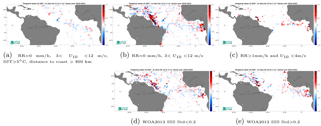
Figure 14: Temporal mean gridded over spatial boxes of size 1^\circ \times 1^\circ of \Delta\text{SSS} (ISAS v7 - Monthly (Ifremer-LOPS-CMEMS) - TSG (GOSUD-Research-vessel)) for 5 different subdatasets corresponding to:RR=0 mm/h, 3 < U_{10} < 12 m/s, SST >5^\circ\text{C} , distance to coast > 800 km (a), RR=0 mm/h, 3 < U_{10} < 12 m/s (b), RR >1 mm/h and U_{10} < 4 m/s (c), WOA2013 SSS Std <0.2 (d), WOA2013 SSS Std >0.2 (e).
