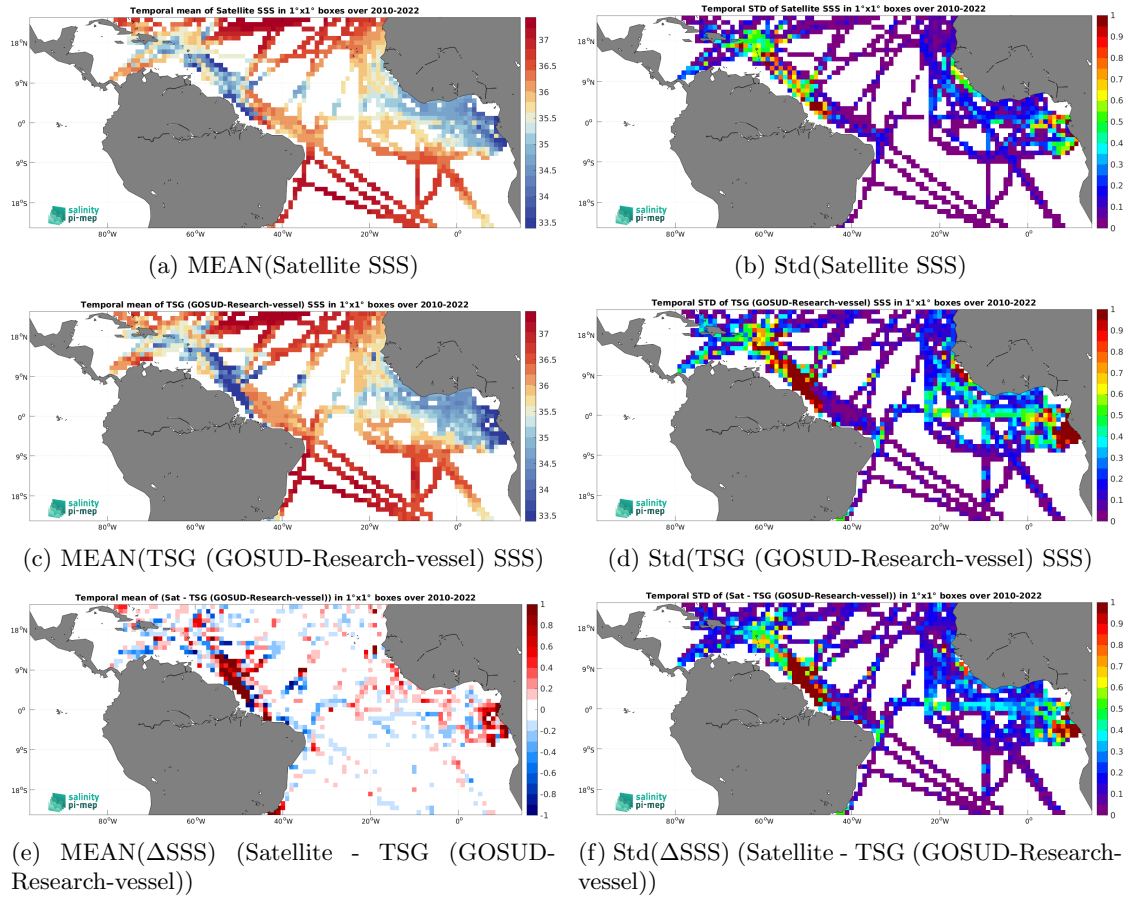
Figure 7: Temporal mean (left) and Std (right) of SSS from ISAS v7 - Monthly (Ifremer-LOPS-CMEMS) (top), TSG (GOSUD-Research-vessel) (middle), and of \Delta SSS (Satellite - TSG (GOSUD-Research-vessel)). Only match-up pairs are used to generate these maps.
