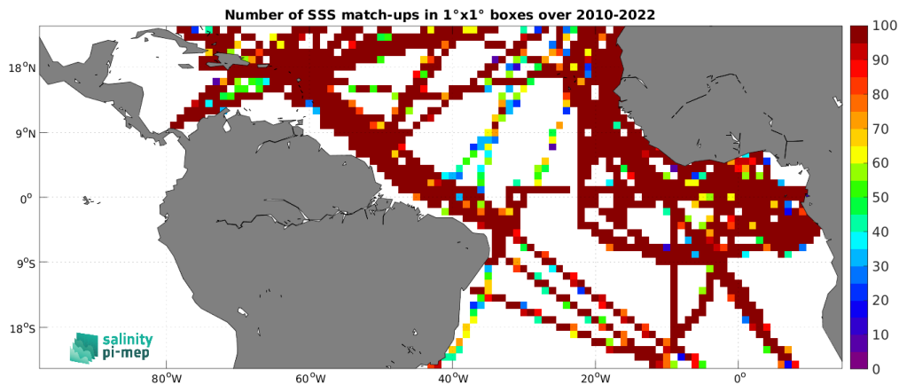
Figure 5: Number of SSS match-ups between TSG (GOSUD-Research-vessel) SSS and the ISAS v7 - Monthly (Ifremer-LOPS-CMEMS) SSS product for the Tropical Atlantic Ocean Pi-MEP region over 1^\circ \times 1^\circ boxes and for the full satellite product period.
