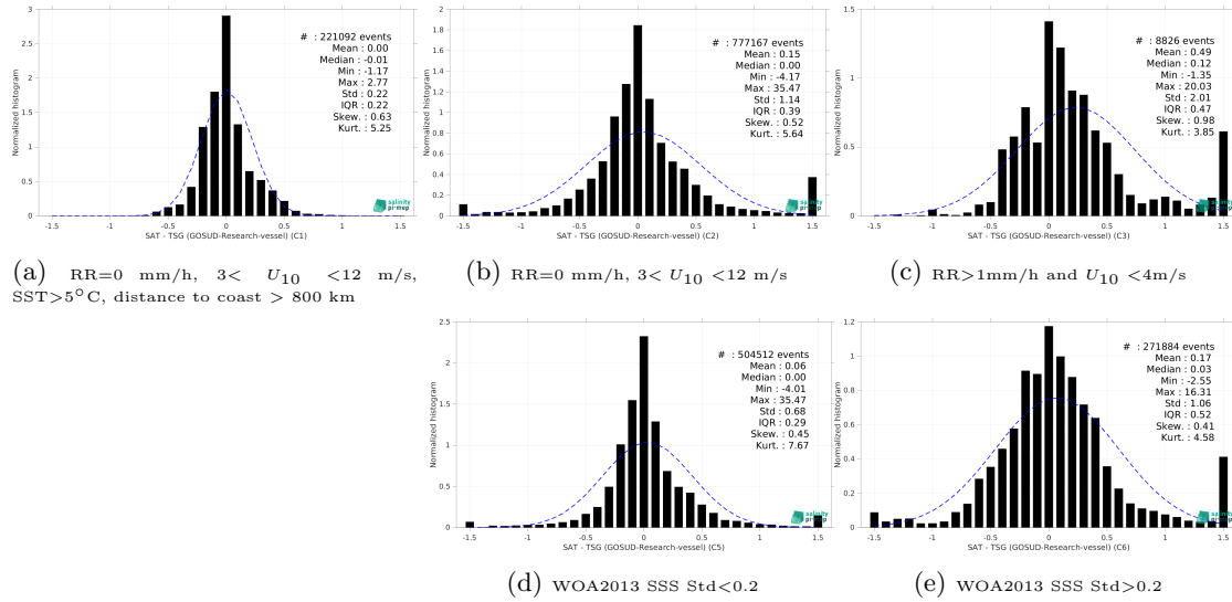
Figure 15: Normalized histogram of \Delta SSS (ISAS v7 - Monthly (Ifremer-LOPS-CMEMS) - TSG (GOSUD-Research-vessel)) for 5 different subdatasets corresponding to: RR=0 mm/h, 3 < U_{10} < 12 m/s, SST>5°C, distance to coast > 800 km (a), RR=0 mm/h, 3 < U_{10} < 12 m/s (b), RR>1mm/h and U_{10} < 4 m/s (c), WOA2013 SSS Std<0.2 (d), WOA2013 SSS Std>0.2 (e).
