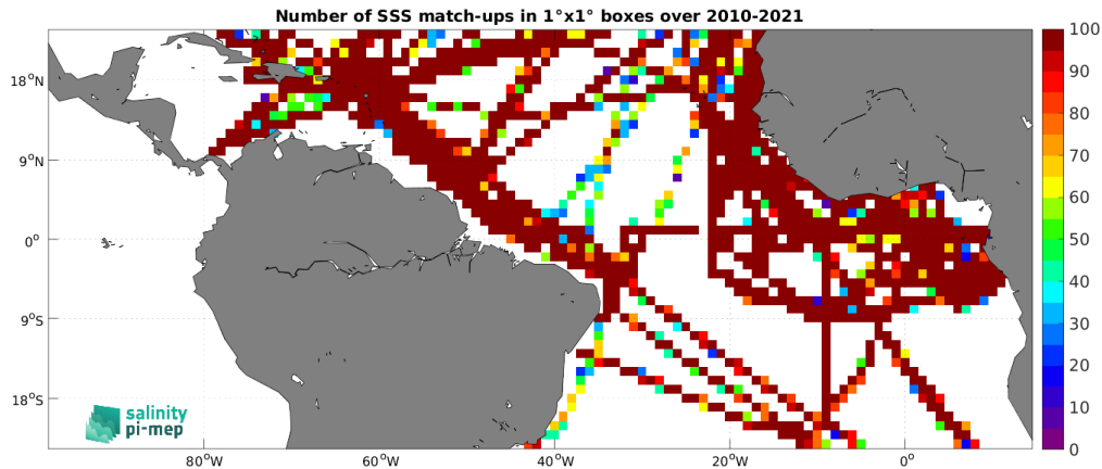
Figure 5: Number of SSS match-ups between TSG (GOSUD-Research-vessel) SSS and the ISAS SSS product for the Tropical Atlantic Ocean Pi-MEP region over 1^\circ \times 1^\circ boxes and for the full satellite product period.
