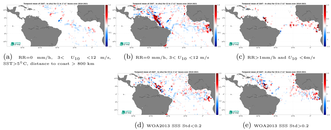
Figure 14: Temporal mean gridded over spatial boxes of size 1^\circ \times 1^\circ of \Delta SSS (ISAS - TSG (GOSUD-Research-vessel)) for 5 different subdatasets corresponding to:RR=0 mm/h, 3 < U_{10} < 12 m/s, SST>5°C, distance to coast > 800 km (a), RR=0 mm/h, 3 < U_{10} < 12 m/s (b), RR>1mm/h and U_{10} < 4 m/s (c), WOA2013 SSS Std<0.2 (d), WOA2013 SSS Std>0.2 (e).
