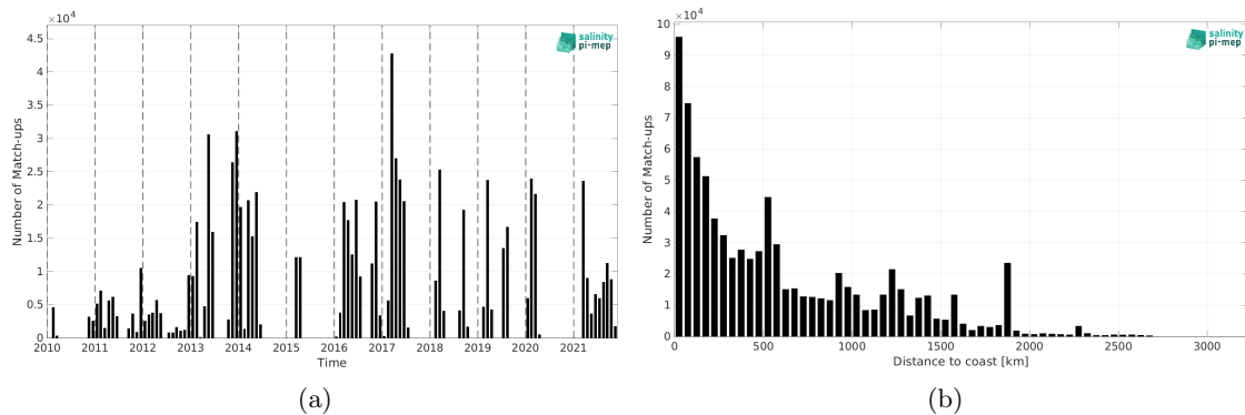
Figure 2: Number of match-ups between TSG (GOSUD-Research-vessel) and ISAS SSS as a function of time (a) and as function of the distance to coast (b) over the Tropical Atlantic Ocean Pi-MEP region and for the full satellite product period.
