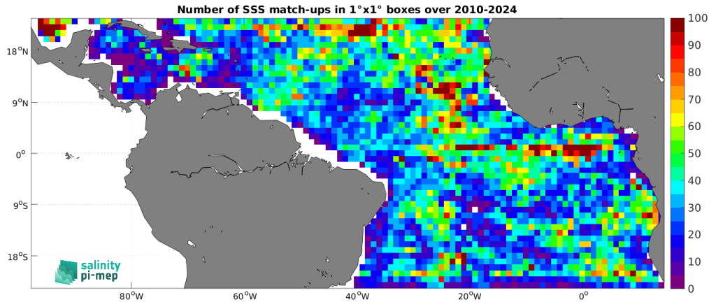
Figure 5: Number of SSS match-ups between Argo SSS and the ISAS v7 - Monthly (Ifremer-LOPS-CMEMS) SSS product for the Tropical Atlantic Ocean Pi-MEP region over 1^\circ \times 1^\circ boxes and for the full satellite product period.
