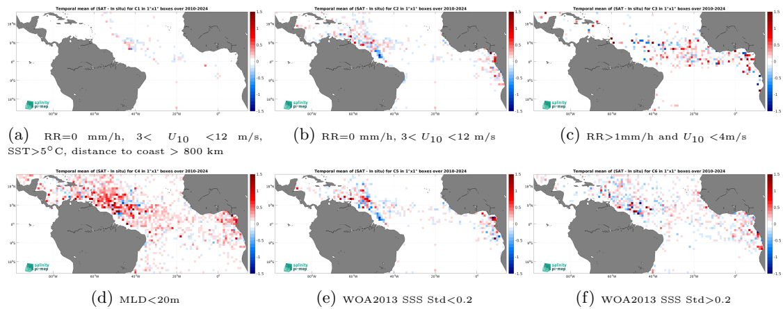
Figure 14: Temporal mean gridded over spatial boxes of size 1^\circ \times 1^\circ of \Delta SSS (ISAS v7 - Monthly (Ifremer-LOPS-CMEMS) - Argo) for 6 different subdatasets corresponding to:RR=0 mm/h, 3 < U_{10} < 12 m/s, SST >5^\circ\text{C} , distance to coast > 800 km (a), RR=0 mm/h, 3 < U_{10} < 12 m/s (b), RR >1 mm/h and U_{10} < 4 m/s (c),MLD <20 m (d),WOA2013 SSS Std <0.2 (e),WOA2013 SSS Std >0.2 (f).
