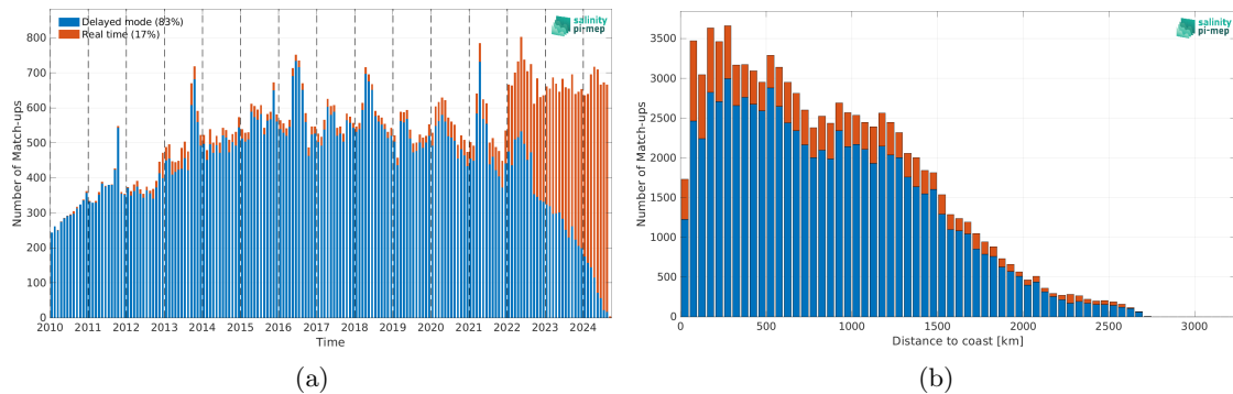
Figure 2: Number of match-ups between Argo and ISAS v7 - Monthly (Ifremer-LOPS-CMEMS) SSS as a function of time (a) and as function of the distance to coast (b) over the Tropical Atlantic Ocean Pi-MEP region and for the full satellite product period.
