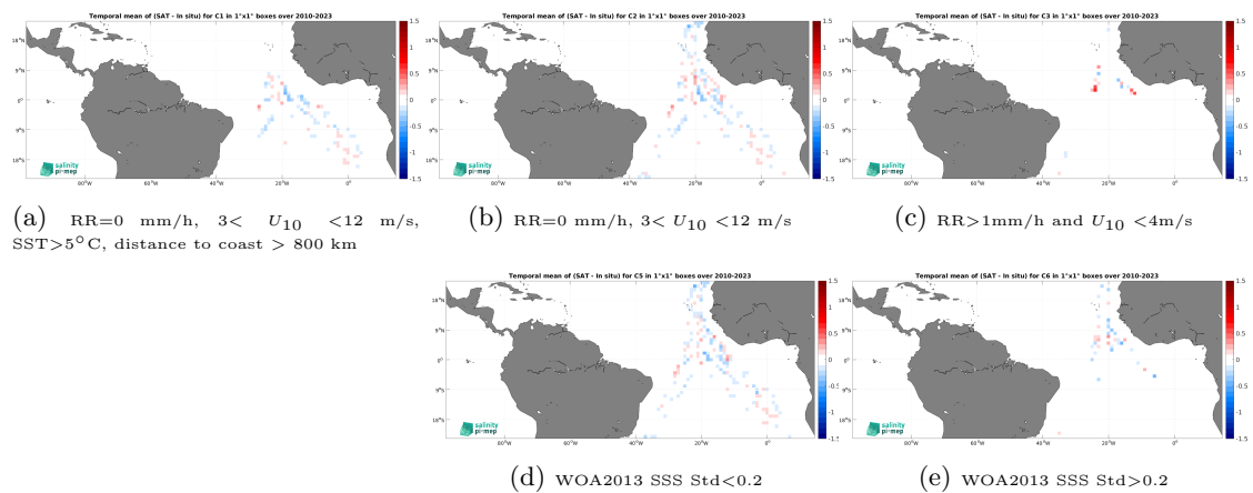
Figure 14: Temporal mean gridded over spatial boxes of size 1^\circ \times 1^\circ of \Delta\text{SSS} (CCI SSS L4 Merged-OI v5.5 - 7-day running (ESA) - TSG (Polarstern)) for 5 different subdatasets corresponding to:RR=0 mm/h, 3 < U_{10} < 12 m/s, SST >5^\circ\text{C} , distance to coast > 800 km (a), RR=0 mm/h, 3 < U_{10} < 12 m/s (b), RR >1 mm/h and U_{10} < 4 m/s (c), WOA2013 SSS Std <0.2 (d), WOA2013 SSS Std >0.2 (e).
