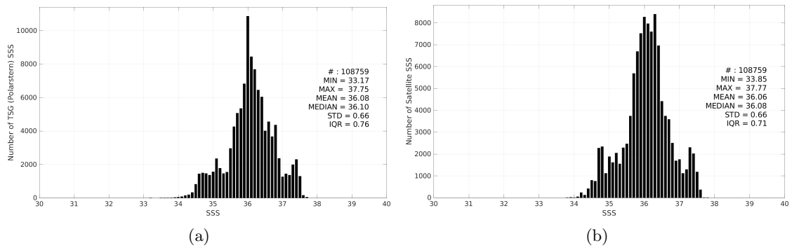
Figure 3: Histograms of SSS from TSG (Polarstern) (a) and CCI SSS L4 Merged-OI v5.5 - 7-day running (ESA) (b) considering all match-up pairs per bins of 0.1 over the Tropical Atlantic Ocean Pi-MEP region and for the full satellite product period.
