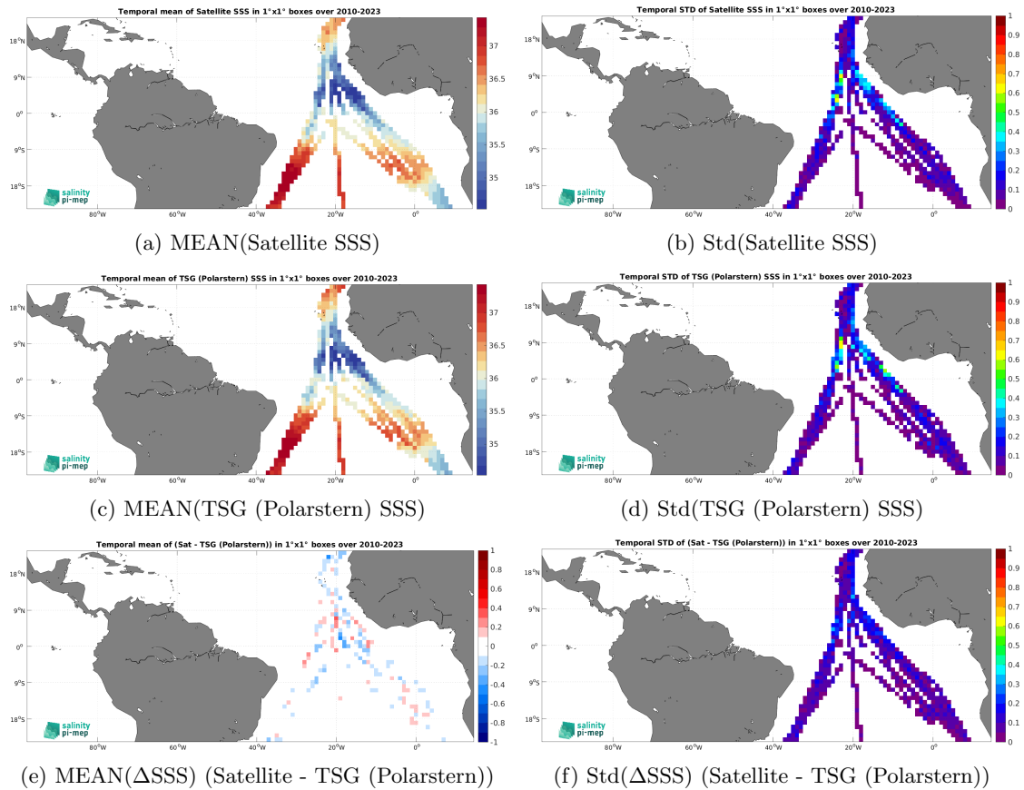
Figure 7: Temporal mean (left) and Std (right) of SSS from CCI SSS L4 Merged-OI v5.5 - 7-day running (ESA) (top), TSG (Polarstern) (middle), and of \Delta SSS (Satellite - TSG (Polarstern)). Only match-up pairs are used to generate these maps.
