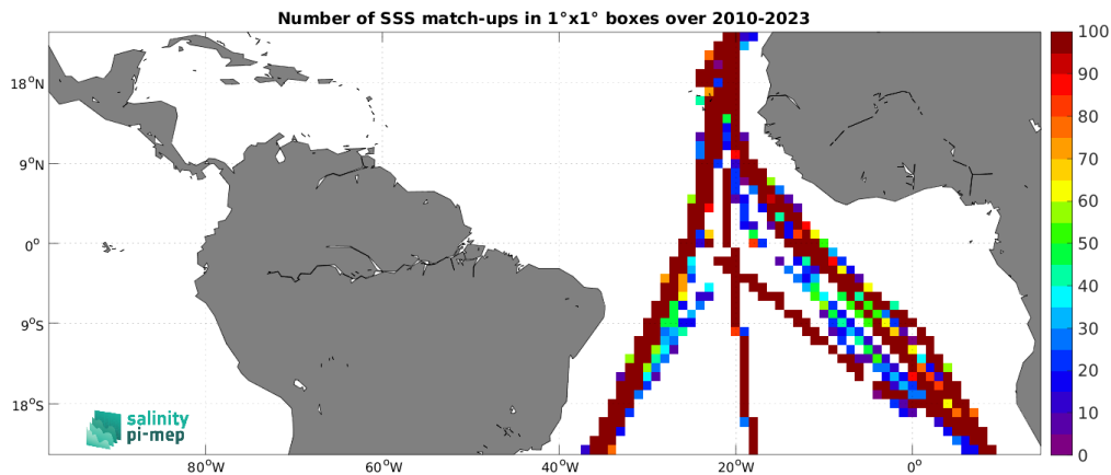
Figure 5: Number of SSS match-ups between TSG (Polarstern) SSS and the CCI SSS L4 Merged-OI v5.5 - 7-day running (ESA) SSS product for the Tropical Atlantic Ocean Pi-MEP region over 1^\circ \times 1^\circ boxes and for the full satellite product period.
