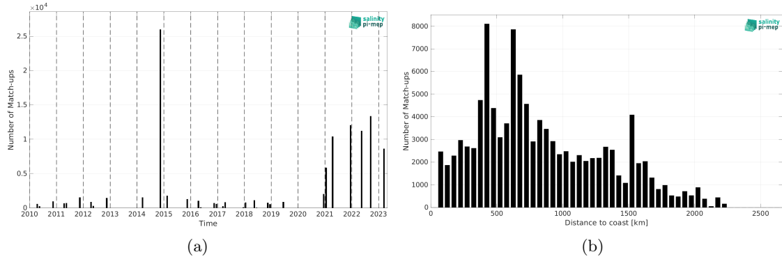
Figure 2: Number of match-ups between TSG (Polarstern) and CCI SSS L4 Merged-OI v5.5 - 7-day running (ESA) SSS as a function of time (a) and as function of the distance to coast (b) over the Tropical Atlantic Ocean Pi-MEP region and for the full satellite product period.
